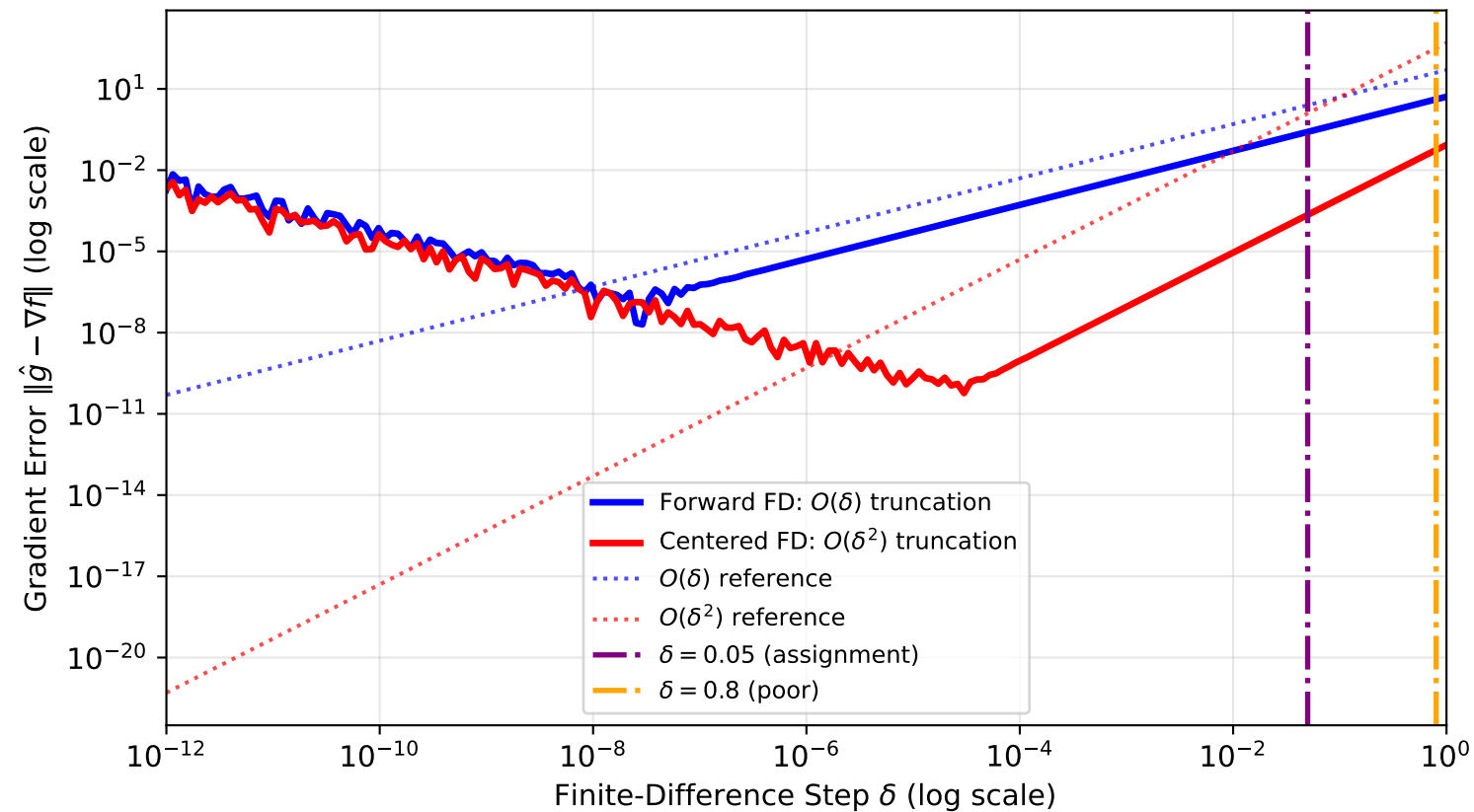
Q4: Forward vs Centered FD Gradient Error (Benchmark B at x_0 = [-1, 4]^T )
