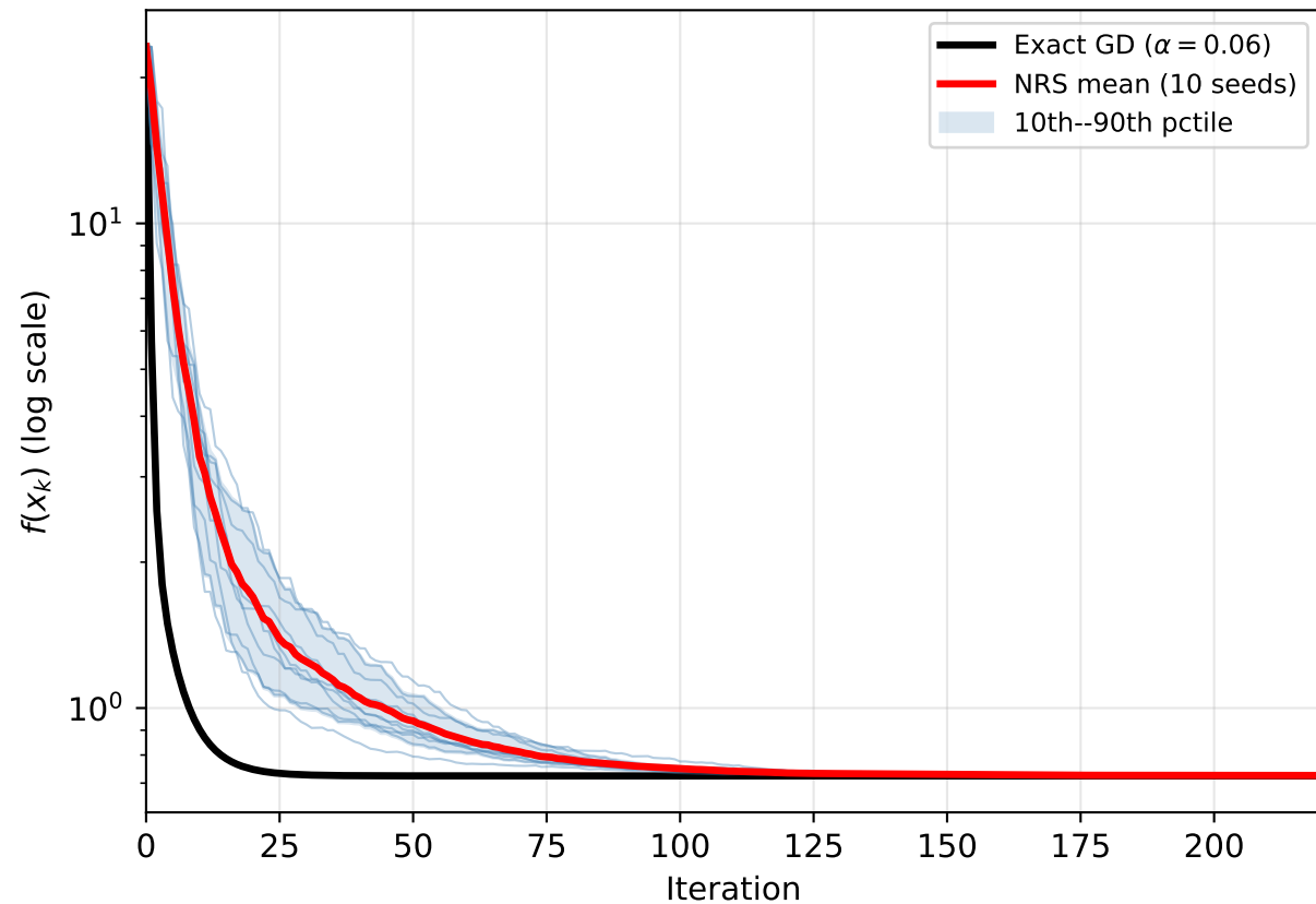
Q4: Nesterov Random Search vs Exact GD (Benchmark B, 10 random seeds)
