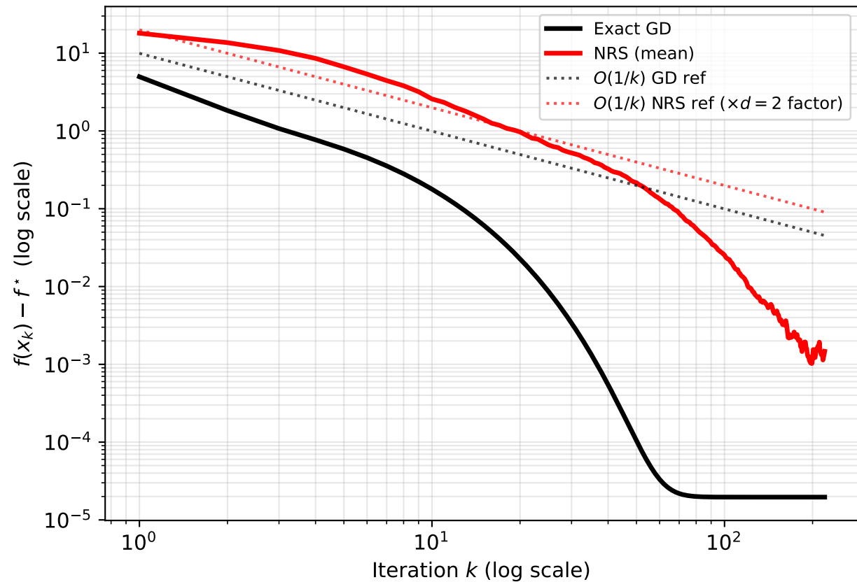
Q4: Convergence Rate Comparison NRS vs GD (Benchmark B, log--log)
