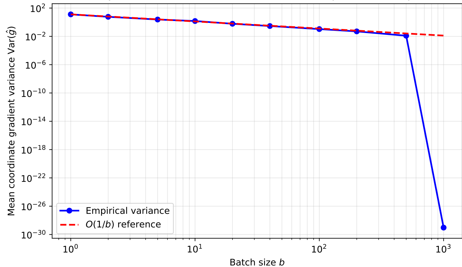
Q2: SGD Gradient Variance vs Batch Size (Benchmark A)
