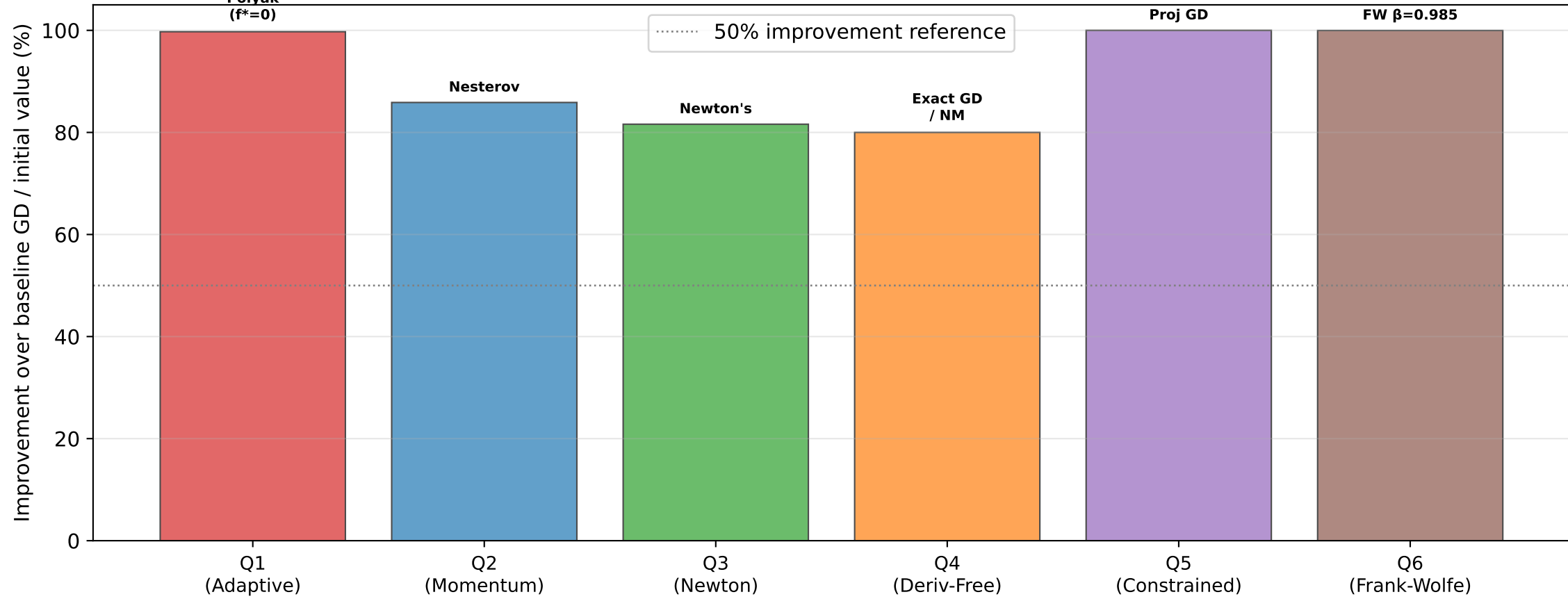
Summary: Best Method Performance Gain by Question (Benchmark C / primary benchmark)
