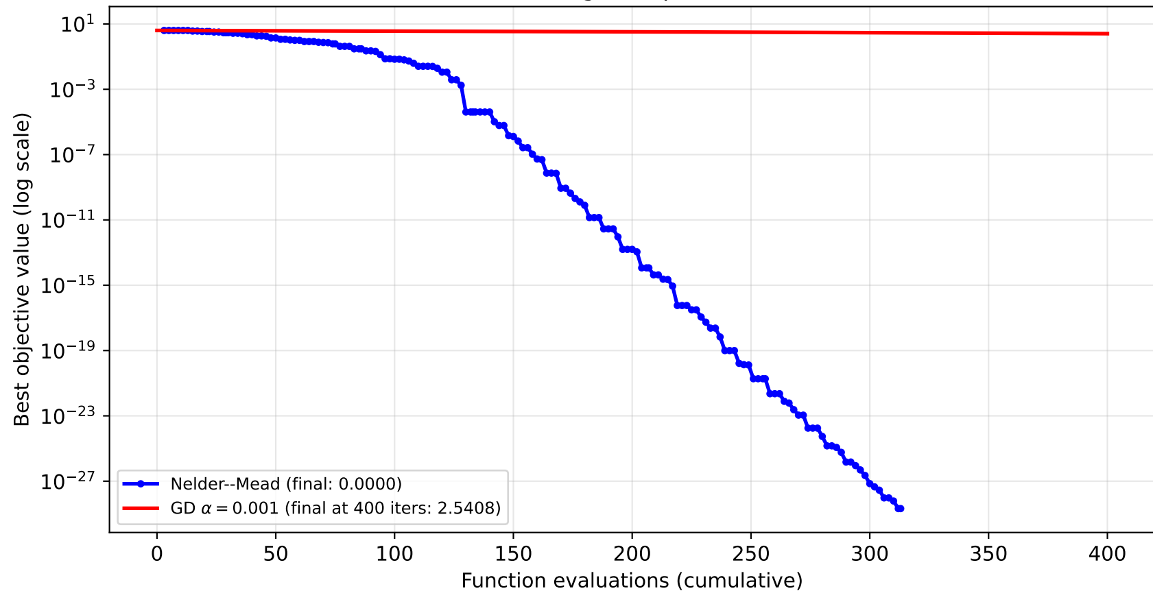
Q4B: Nelder--Mead vs GD — Convergence per Function Evaluation (Rosenbrock)
