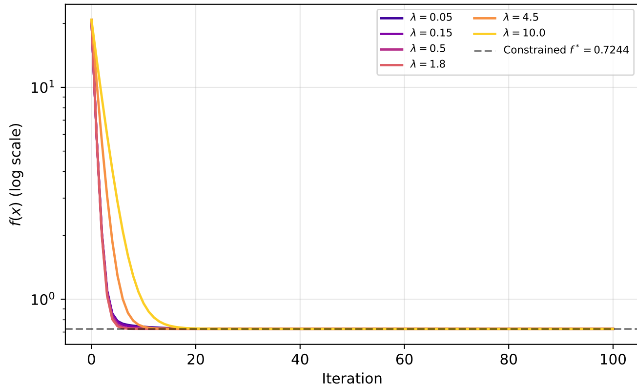
Q5: Penalty Method Sensitivity to \lambda (Step Sizes Adjusted)
