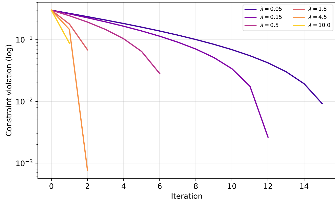
Q5: Constraint Violation vs \lambda
