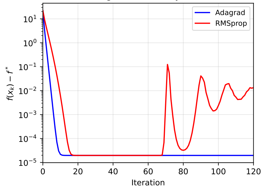
Convergence on Benchmark B (Adagrad eventually stalls)
