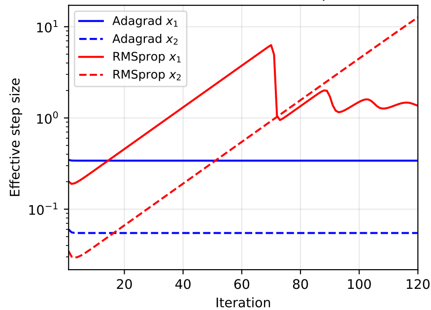
Per-coordinate step sizes (Benchmark B, anisotropic)
