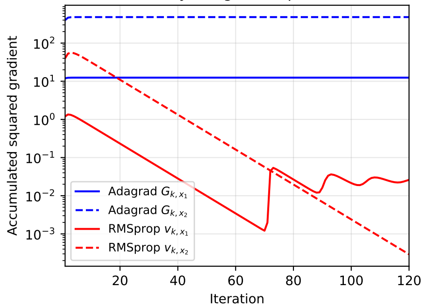
G_k (Adagrad) vs v_k (RMSprop) shows why Adagrad step vanishes
