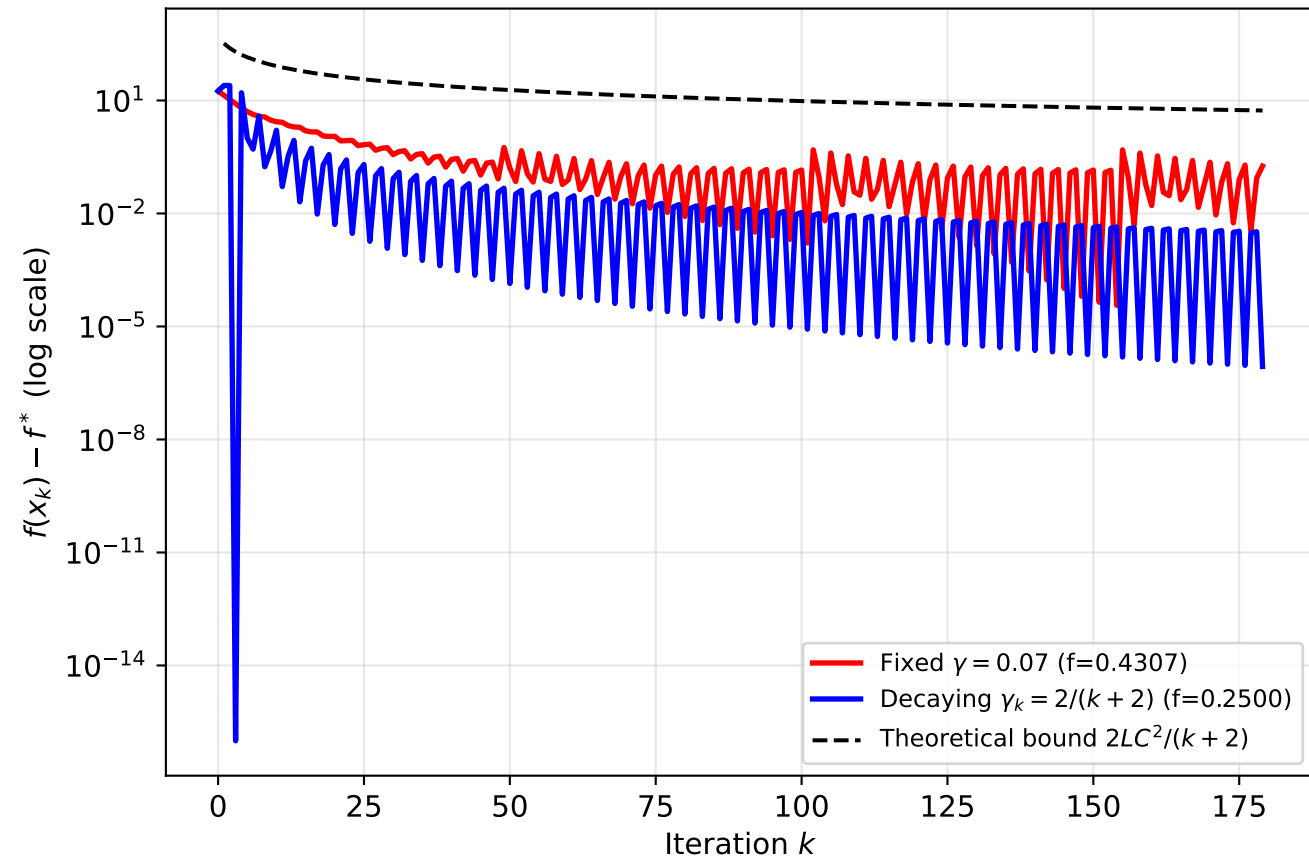
Q6: FW Fixed vs Decaying Step (boundary case)
