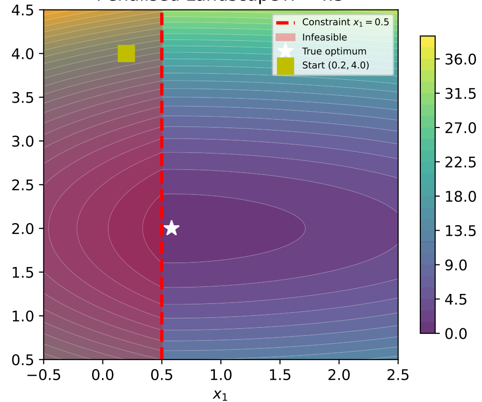
Penalised Landscape \lambda = 4.5
