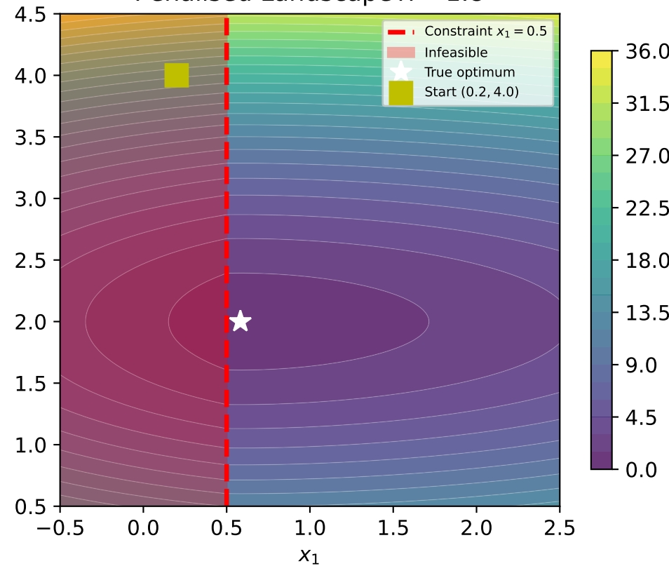
Penalised Landscape \lambda = 1.8
