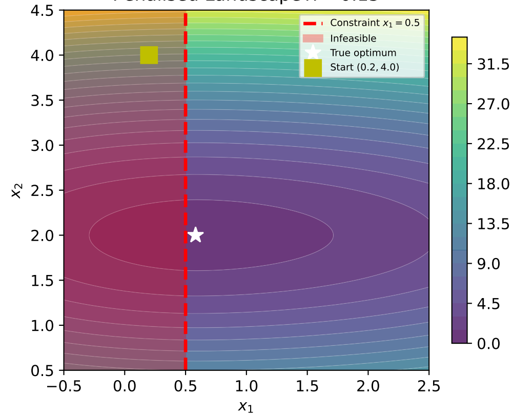
Penalised Landscape \lambda = 0.15
