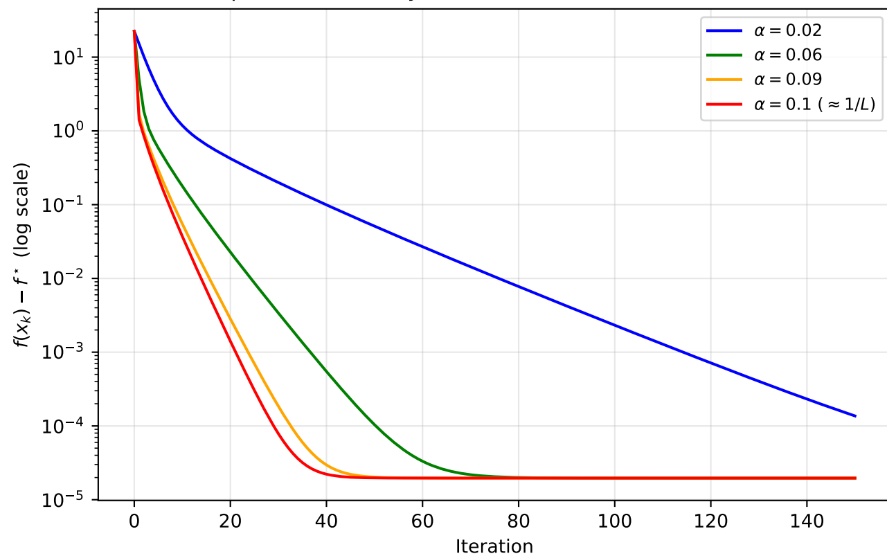
GD Step-Size Sensitivity on Benchmark B ( \kappa \approx 6.90 , 1/L = 0.1 )
