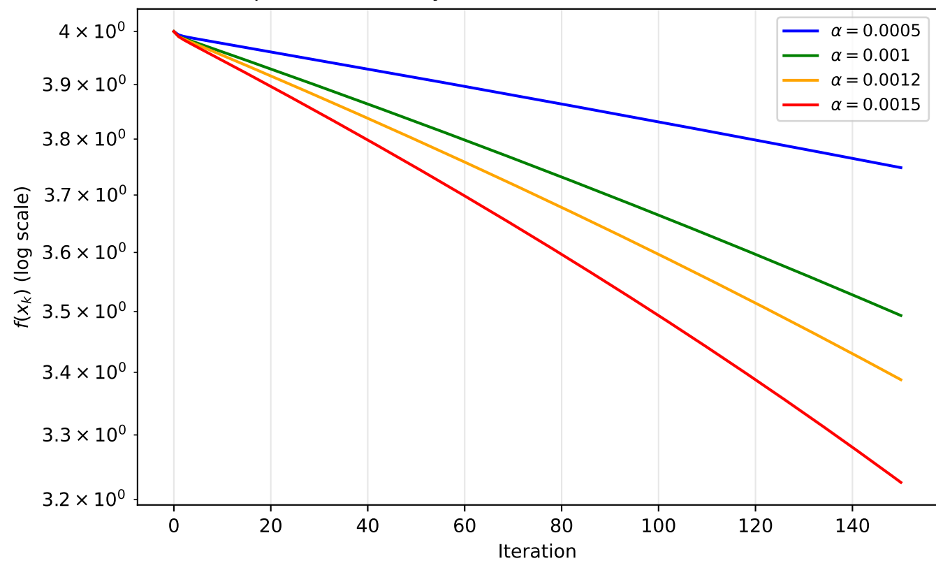
GD Step-Size Sensitivity on Benchmark C ( \kappa \approx 2508 , 1/L \approx 0.001 )
