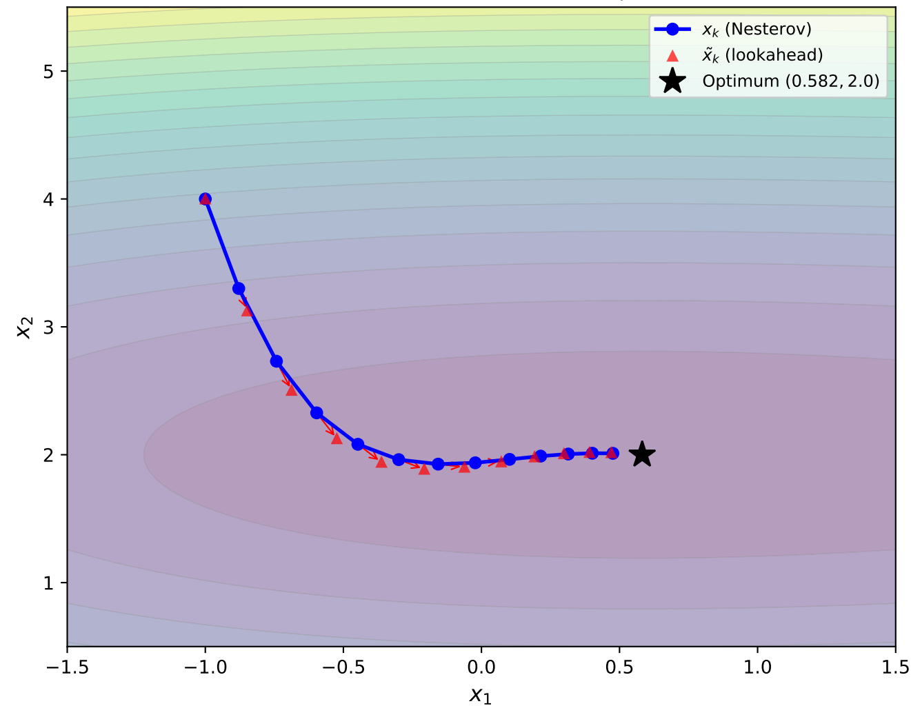
Nesterov momentum: x_k vs lookahead \tilde{x}_k (arrows show momentum step)
