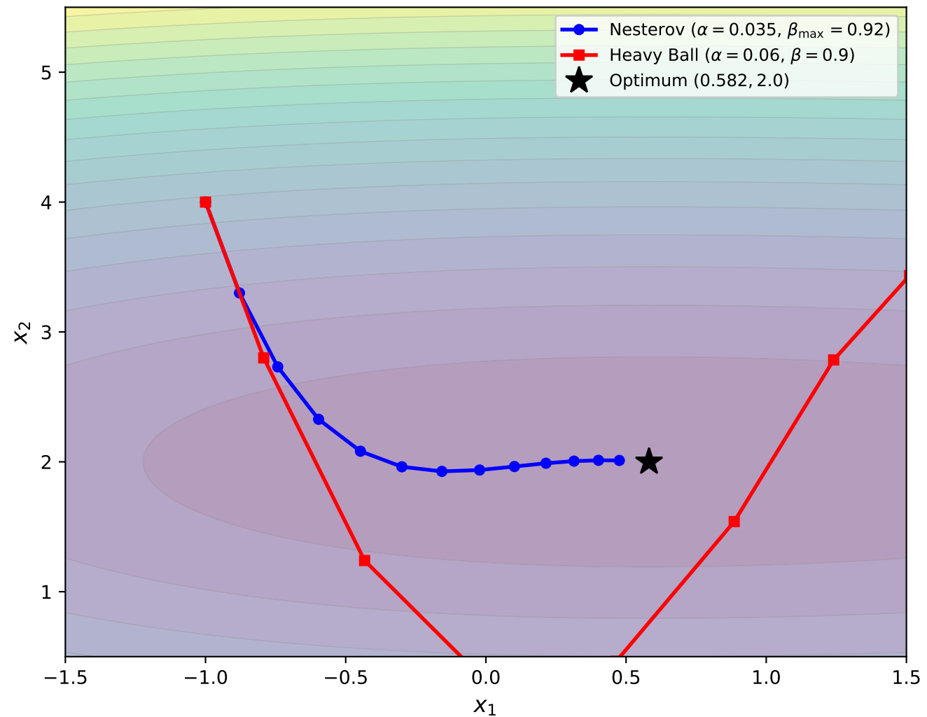
Nesterov vs Heavy Ball (12 iterations) on Benchmark B
