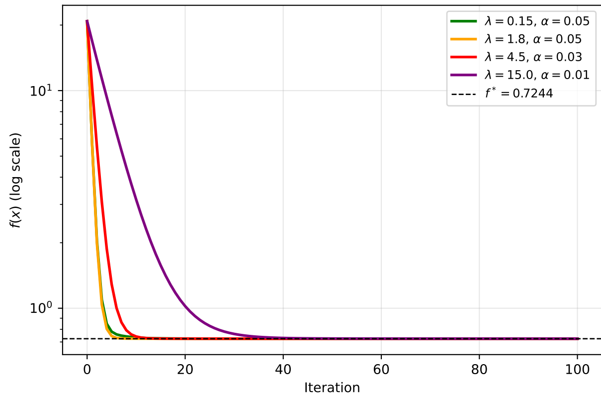
Q5: Penalty Method — Objective vs \lambda
