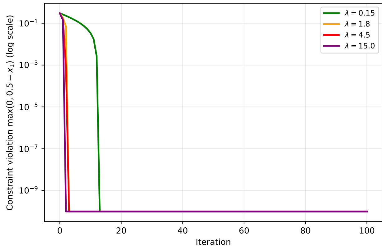
Q5: Penalty Method — Constraint Violation vs \lambda
