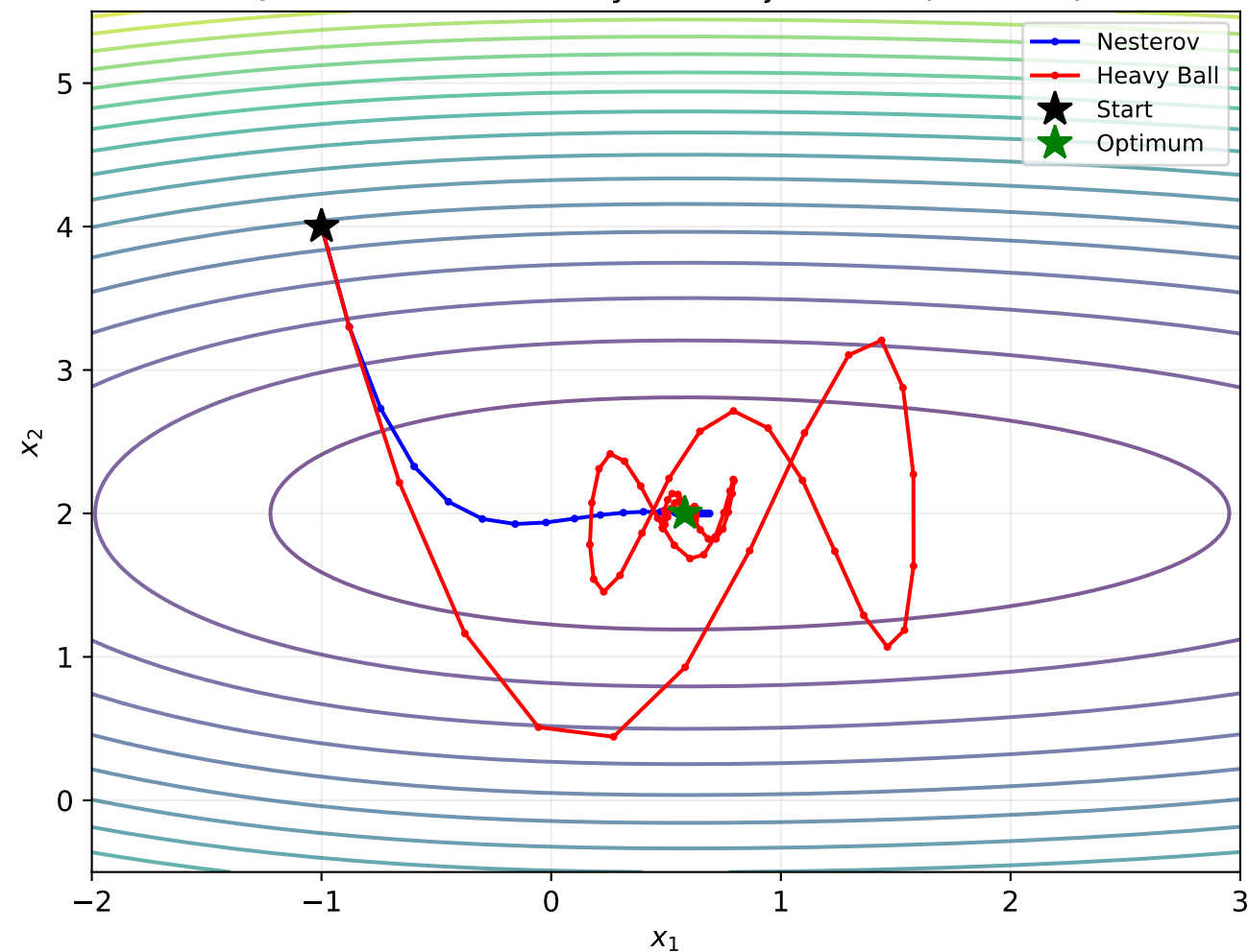
Q2: Nesterov vs Heavy Ball Trajectories (Bench B)
