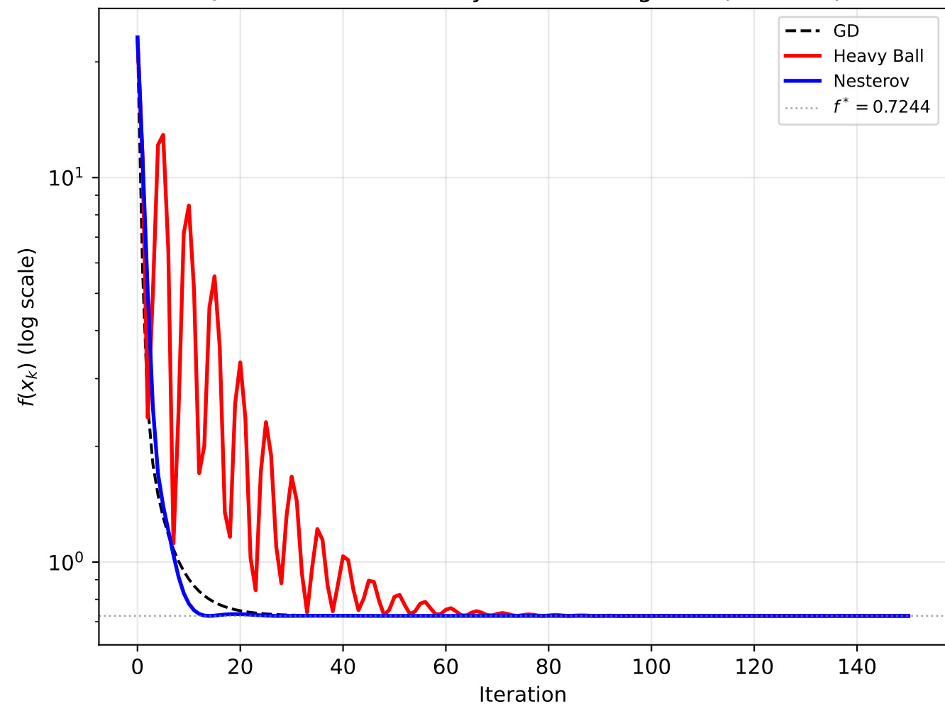
Q2: Nesterov vs Heavy Ball Convergence (Bench B)
