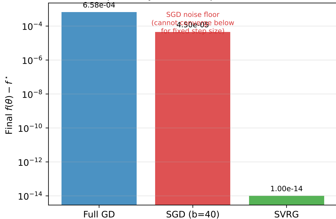
Final suboptimality after 60 epochs on Benchmark A
