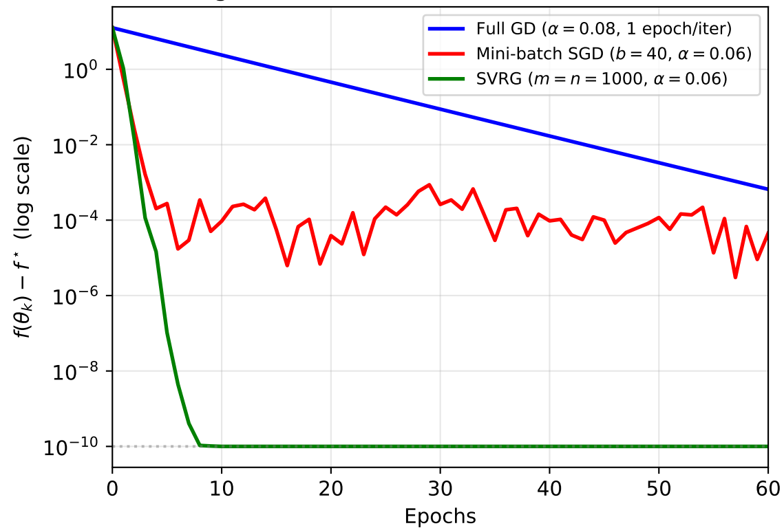
Convergence on Benchmark A: GD vs SGD vs SVRG
