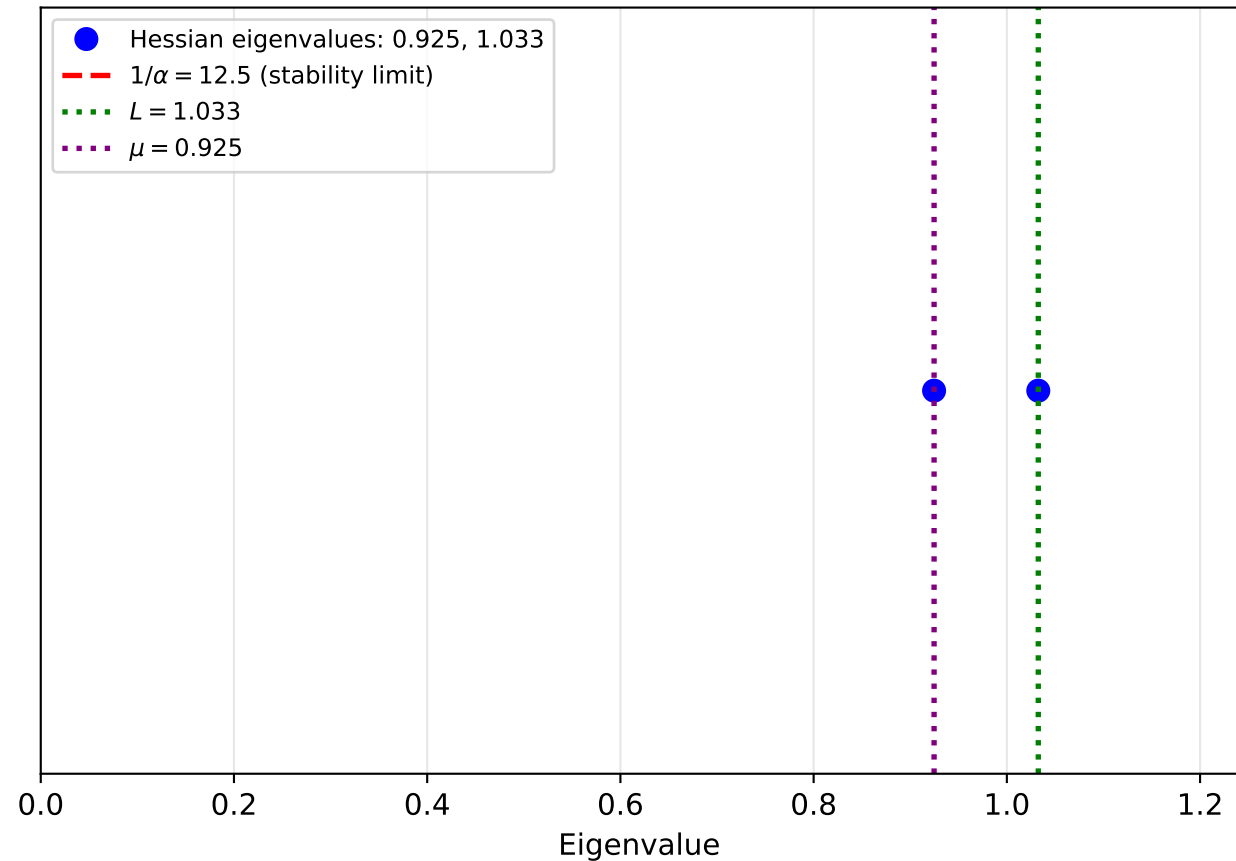
Benchmark A Hessian Spectrum ( \kappa = L/\mu = 1.1 )
