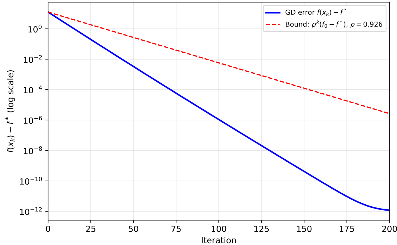
GD Linear Convergence on Benchmark A ( \kappa = 1.1 , \alpha = 0.08 )
