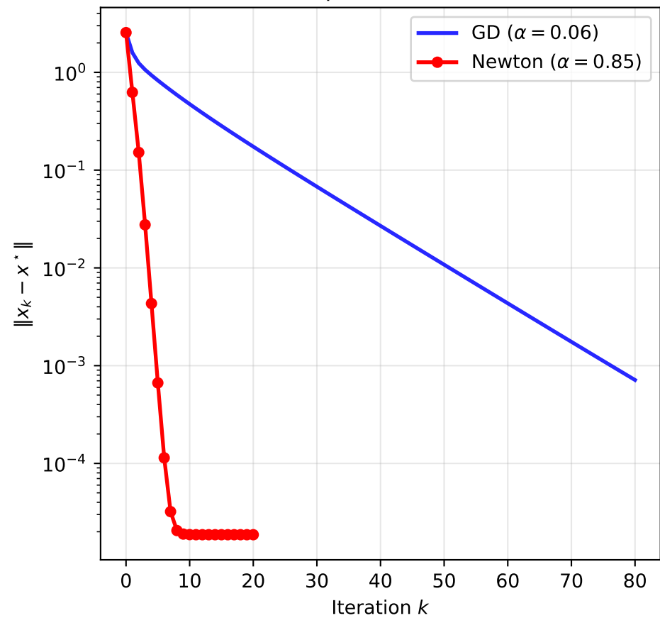
Distance to Optimum (Benchmark B)
