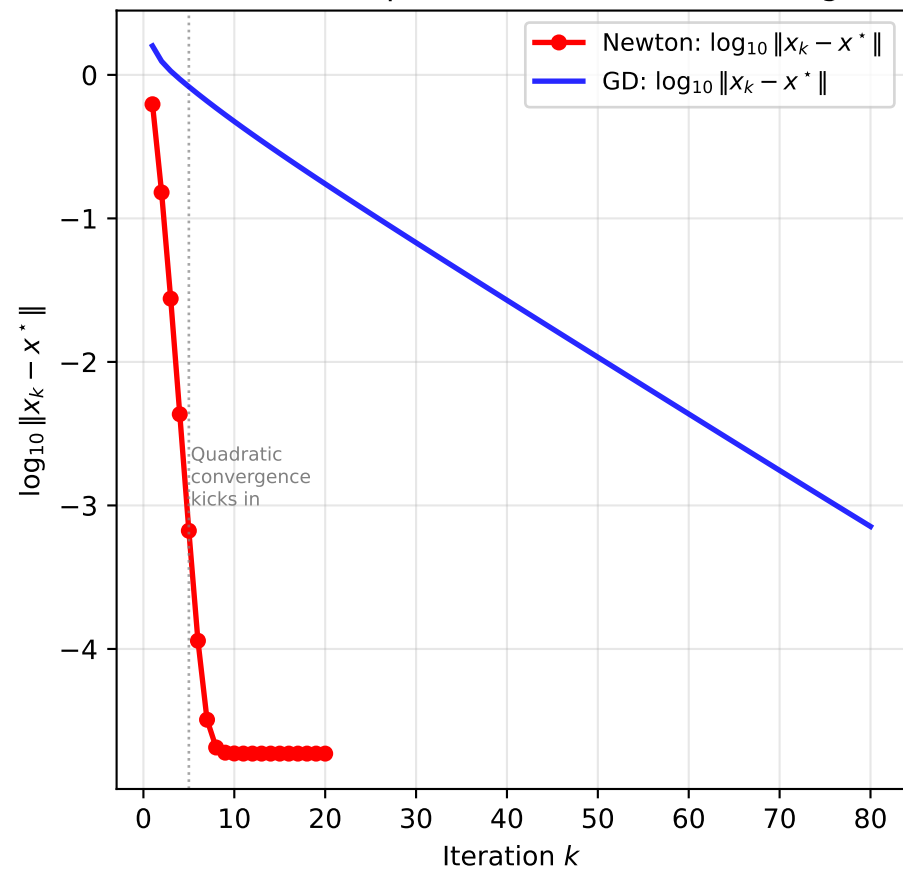
Linear (GD) vs Super-linear (Newton) Convergence
