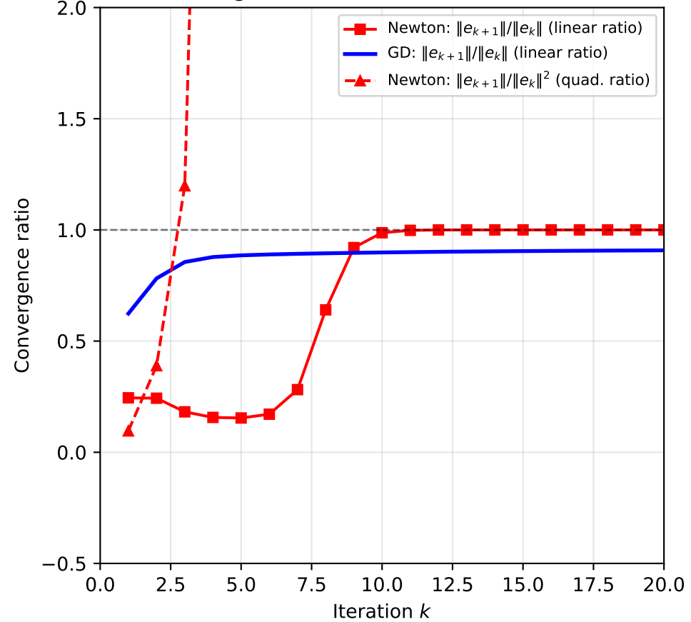
Convergence Order: Linear vs Quadratic
