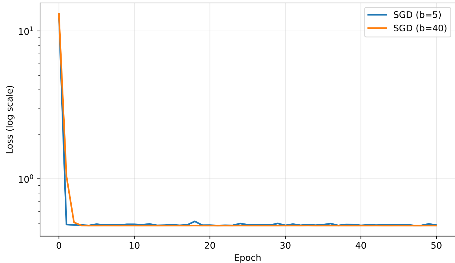
Q2: Mini-Batch SGD — Effect of Batch Size (Benchmark A)
