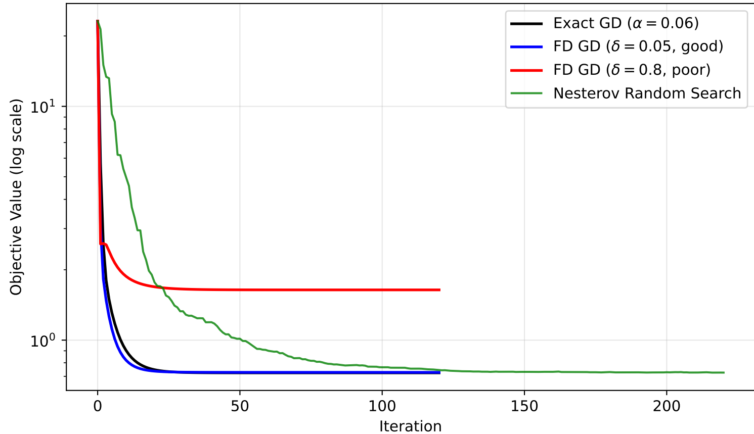
Q4A: Derivative Approximation Methods — Benchmark B
