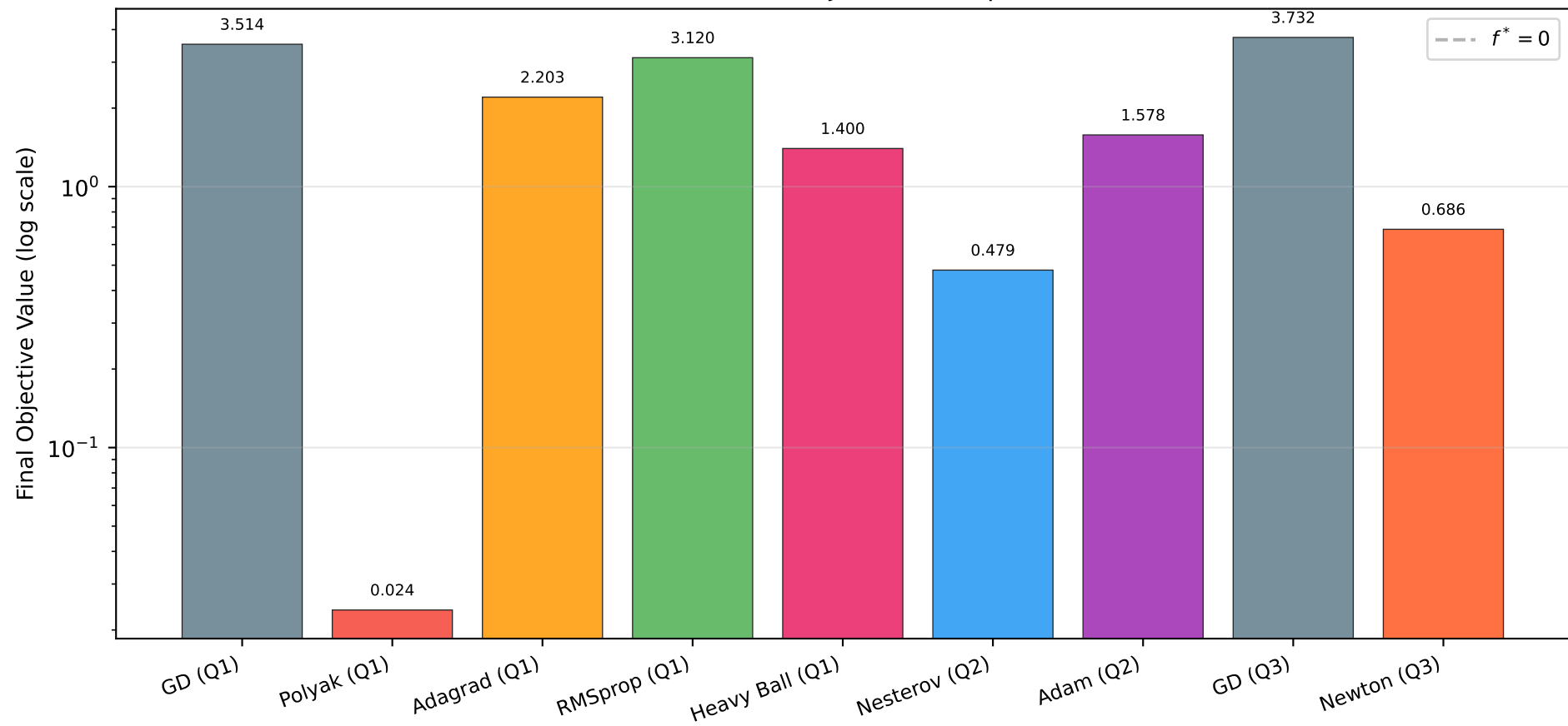
Benchmark C (Rosenbrock): Final Objective Comparison Across All Methods
