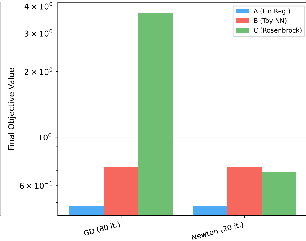
Q3: GD (80 it.) vs Newton (20 it.)
