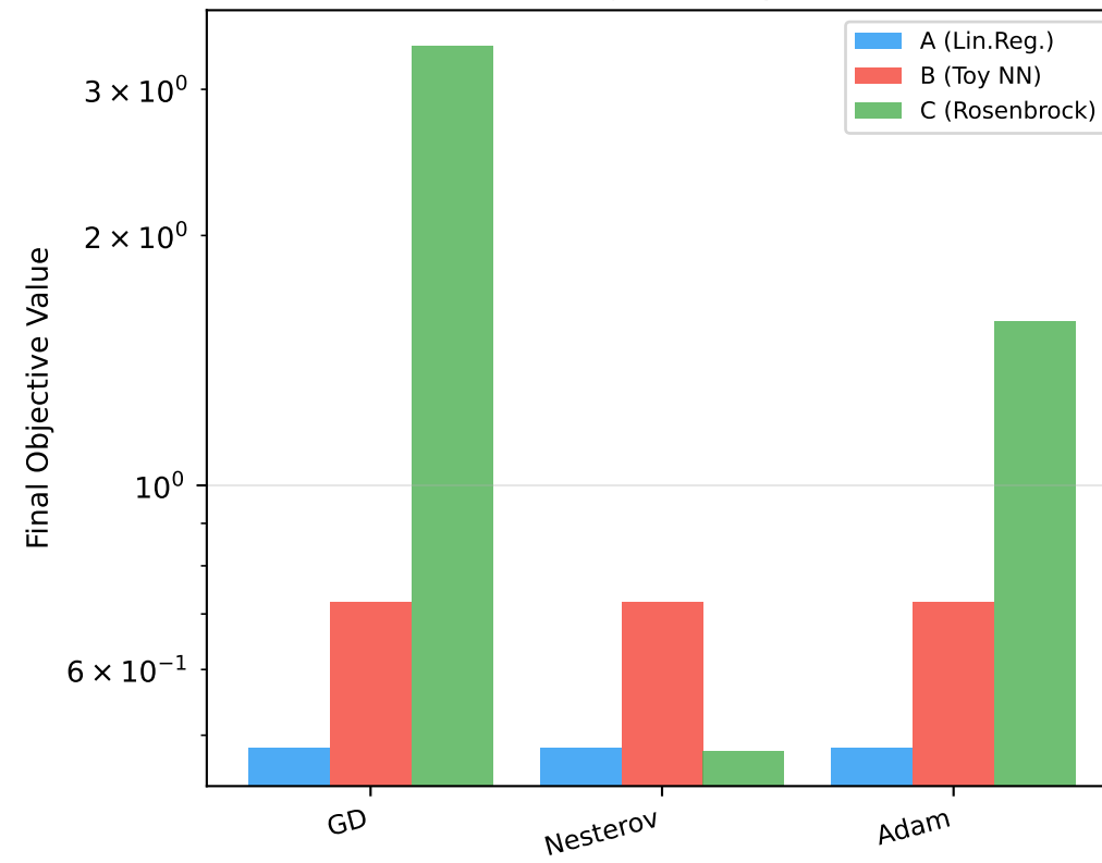
Q2: Final Objective by Method
