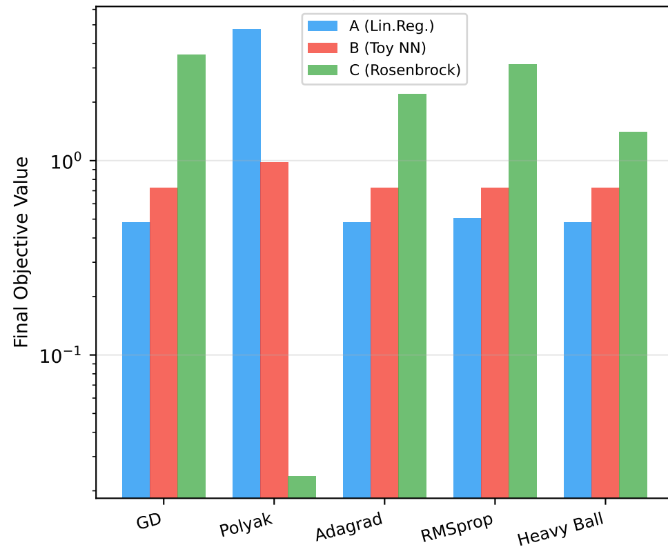
Q1: Final Objective by Method
