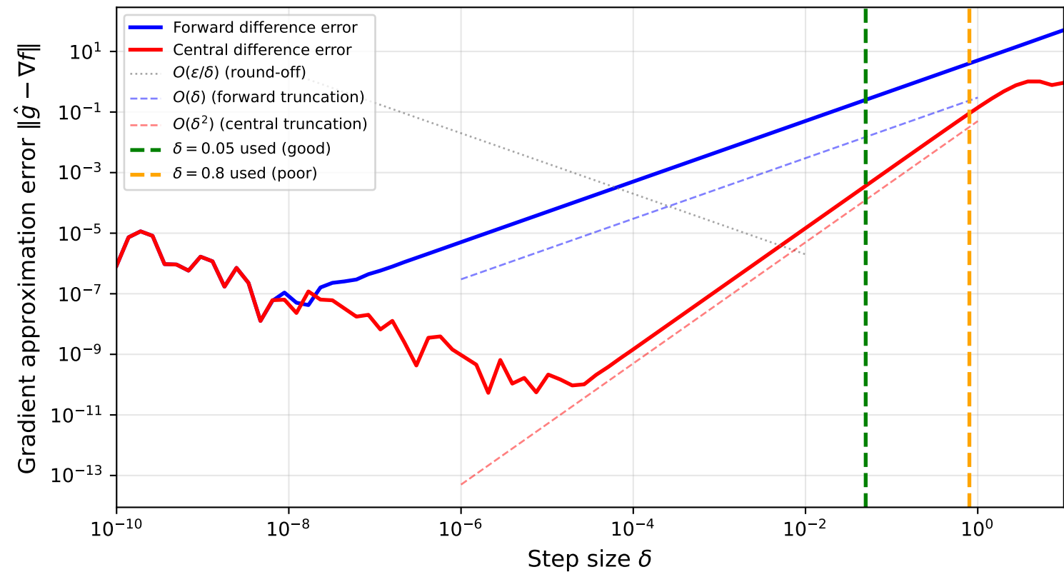
Q4: Finite Difference Gradient Error vs. Step Size \delta Benchmark B evaluated at x = (0.5, 3.0)
