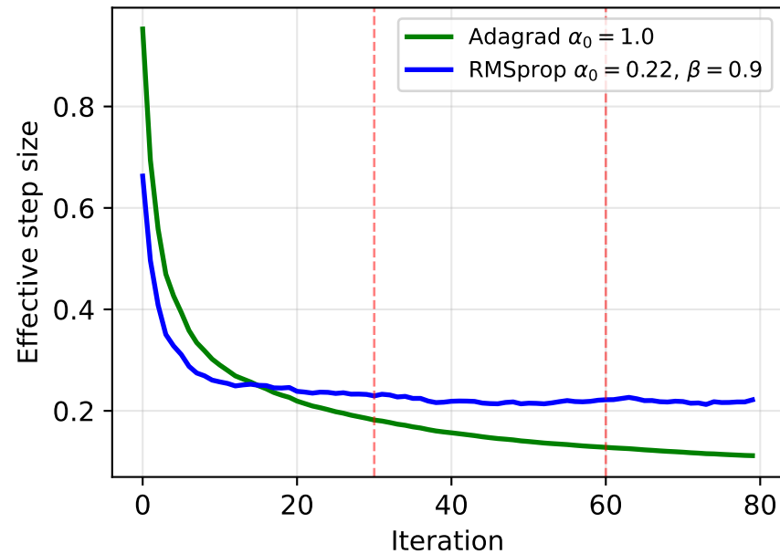
Effective Step Size: Memory Effect
