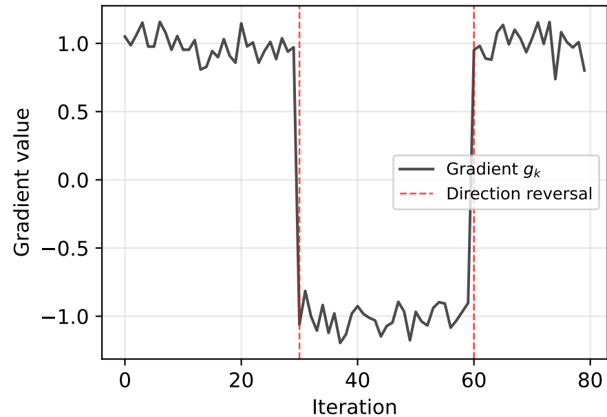
Gradient sequence (direction reversal at k=30,60)
