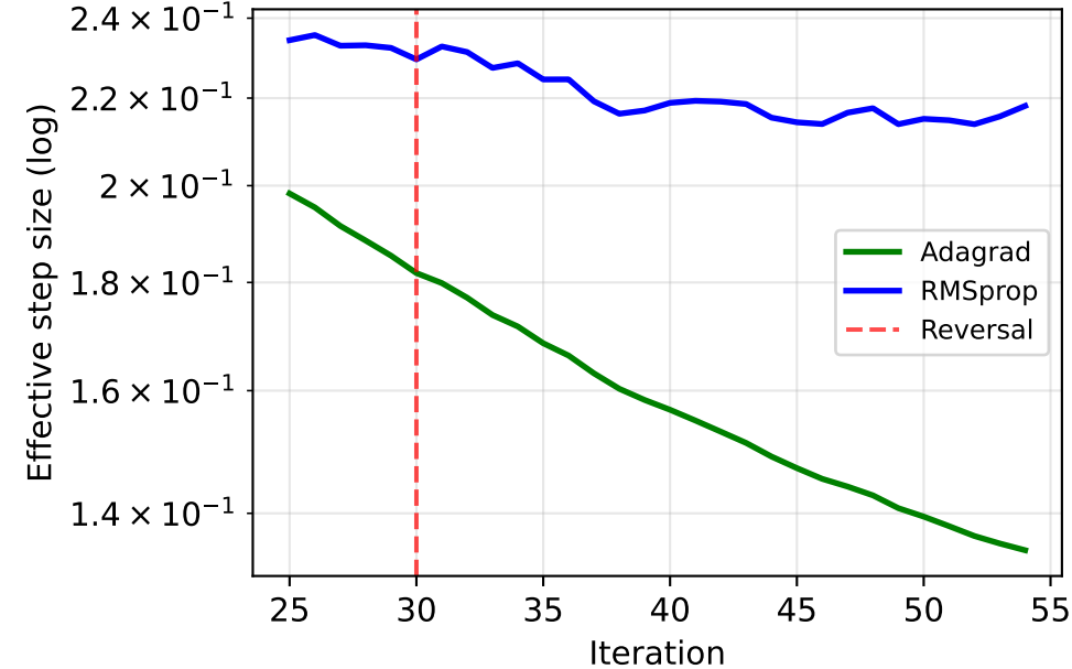
Zoom: Step recovery after reversal (k=25-55)
