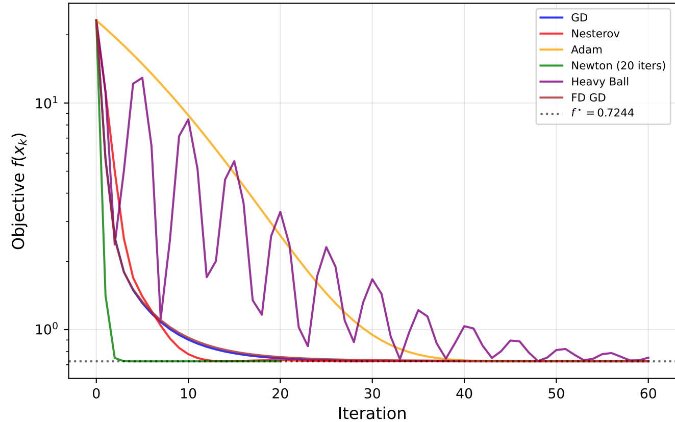
Convergence Comparison on Benchmark B (first 60 iterations)
