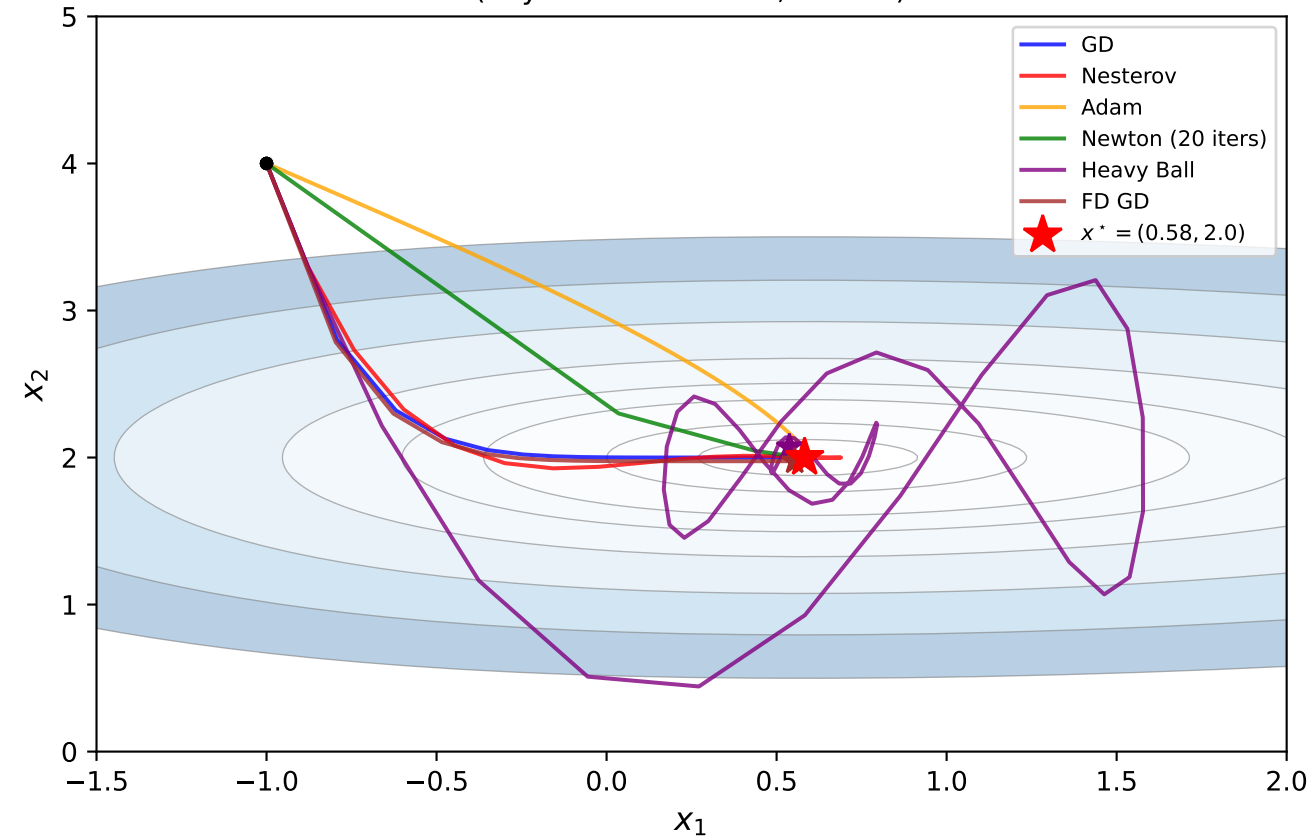
All Method Trajectories on Benchmark B (Toy Neural Network, \kappa \approx 6.9 )
