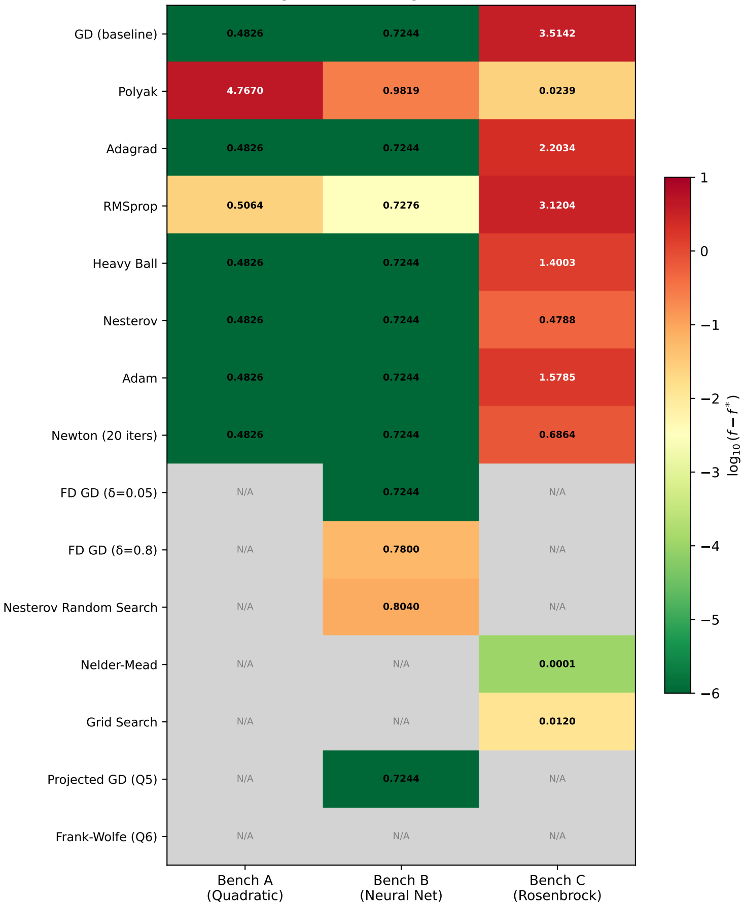
Sub-optimality Heatmap \log_{10}(f(x_k) - f^*) (green = better)
