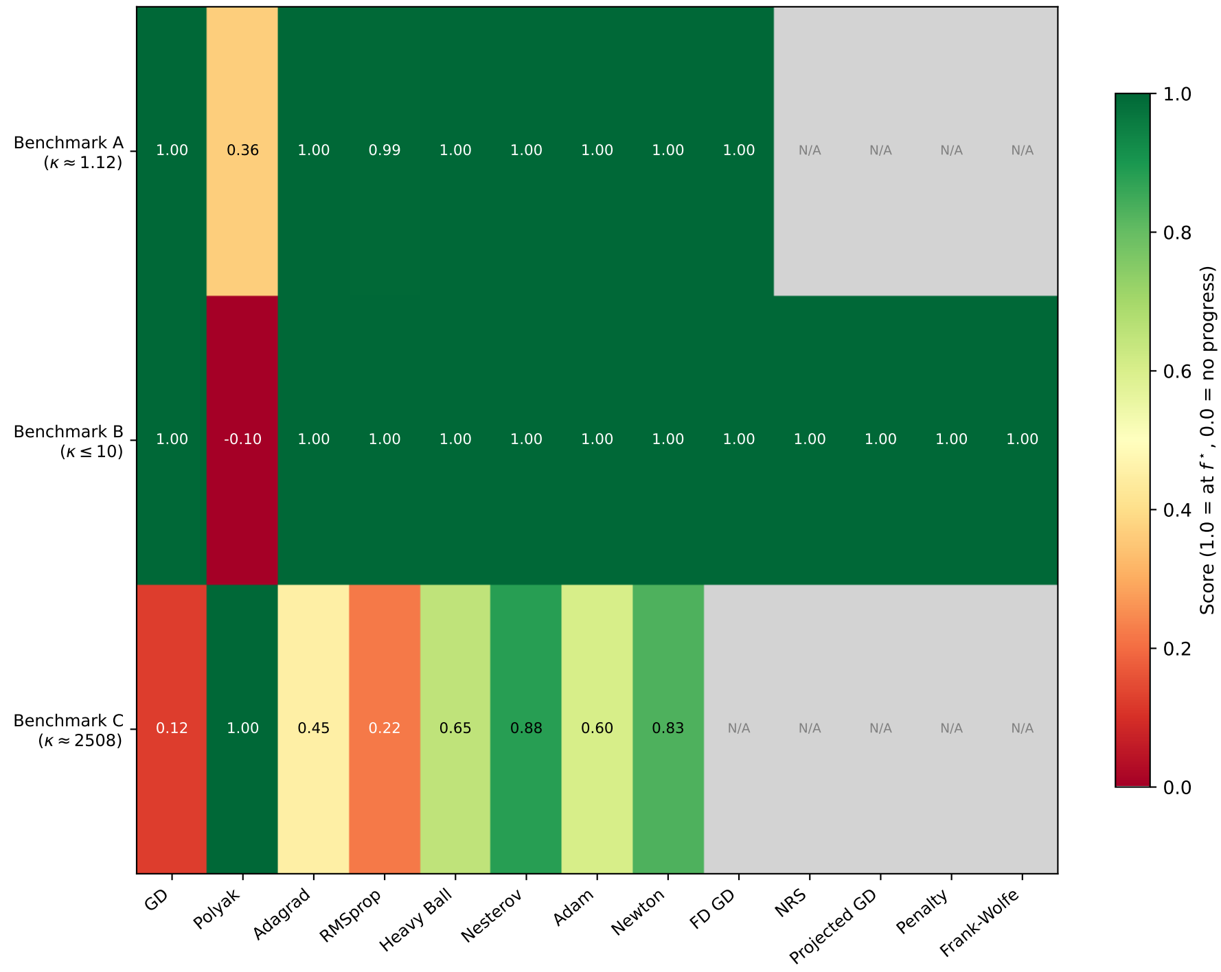
Method Performance Heatmap: Score = 1 - (f_{\text{final}} - f^*) / (f_0 - f^*) (1.0 = perfect convergence, gray = not applicable, negative = diverged)
