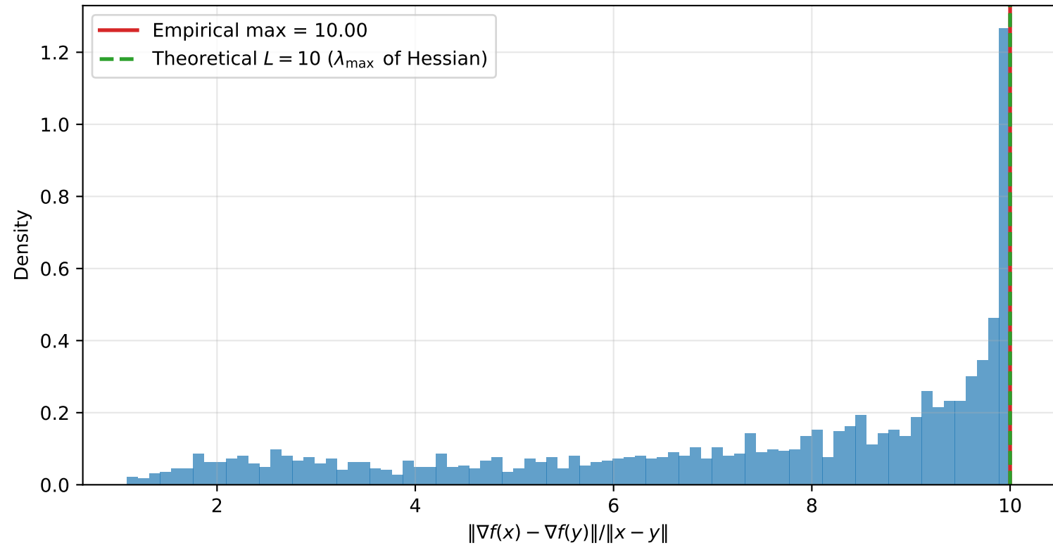
Empirical Lipschitz Constant Distribution for Benchmark B on [-2, 3] \times [-2, 5]
