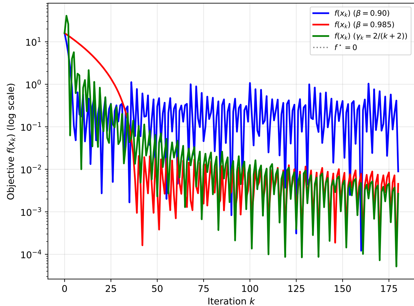
Q6: FW Objective — Fixed \beta vs Standard Step
