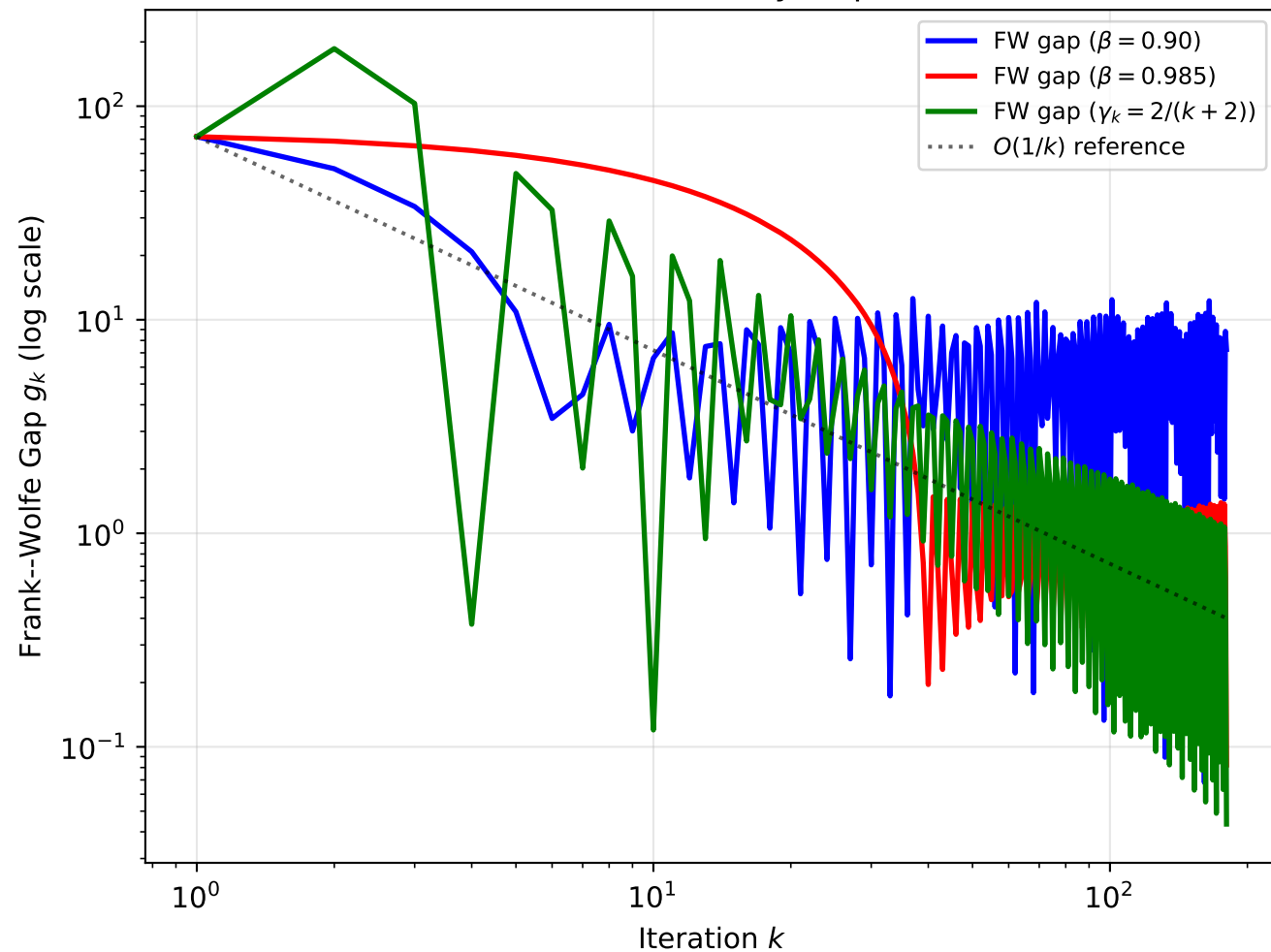
Q6: Frank--Wolfe Duality Gap Evolution
