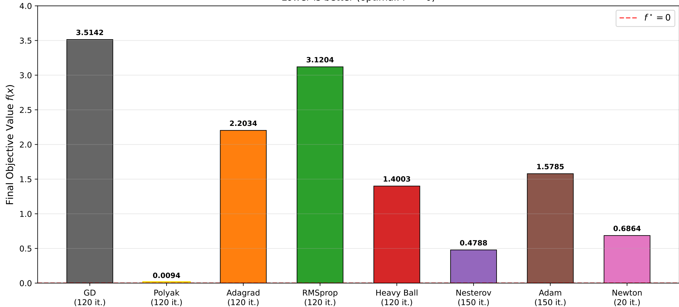
Benchmark C (Rosenbrock): Final Objective Value Comparison Lower is better (optimal: f^* = 0 )
