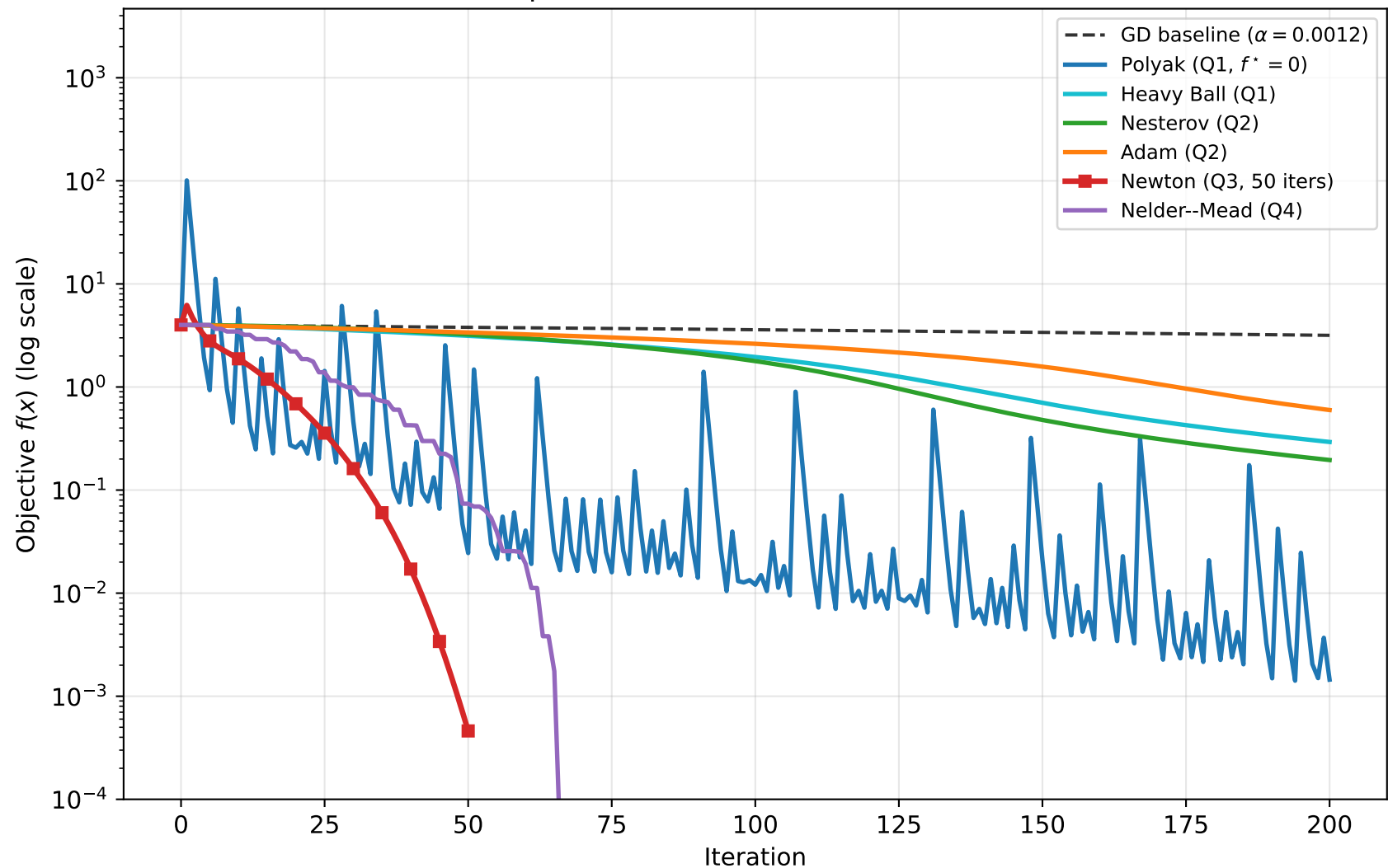
Cross-Question Comparison: All Methods on Rosenbrock (Benchmark C)
