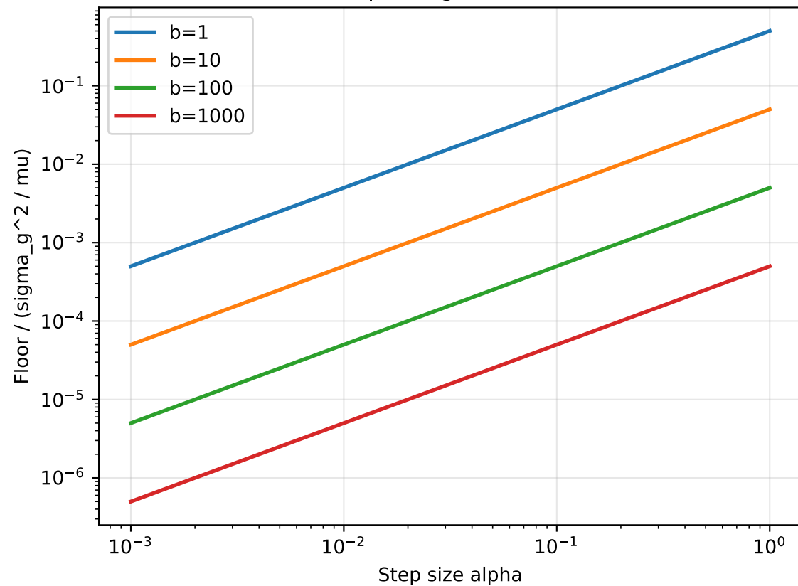
SGD Convergence Floor vs Step Size (floor = \alpha \cdot \sigma^2 / (2 \cdot \mu \cdot b) )
