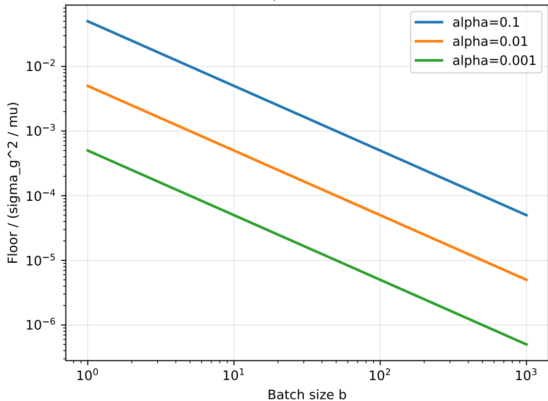
SGD Convergence Floor vs Batch Size (linear improvement with b )
