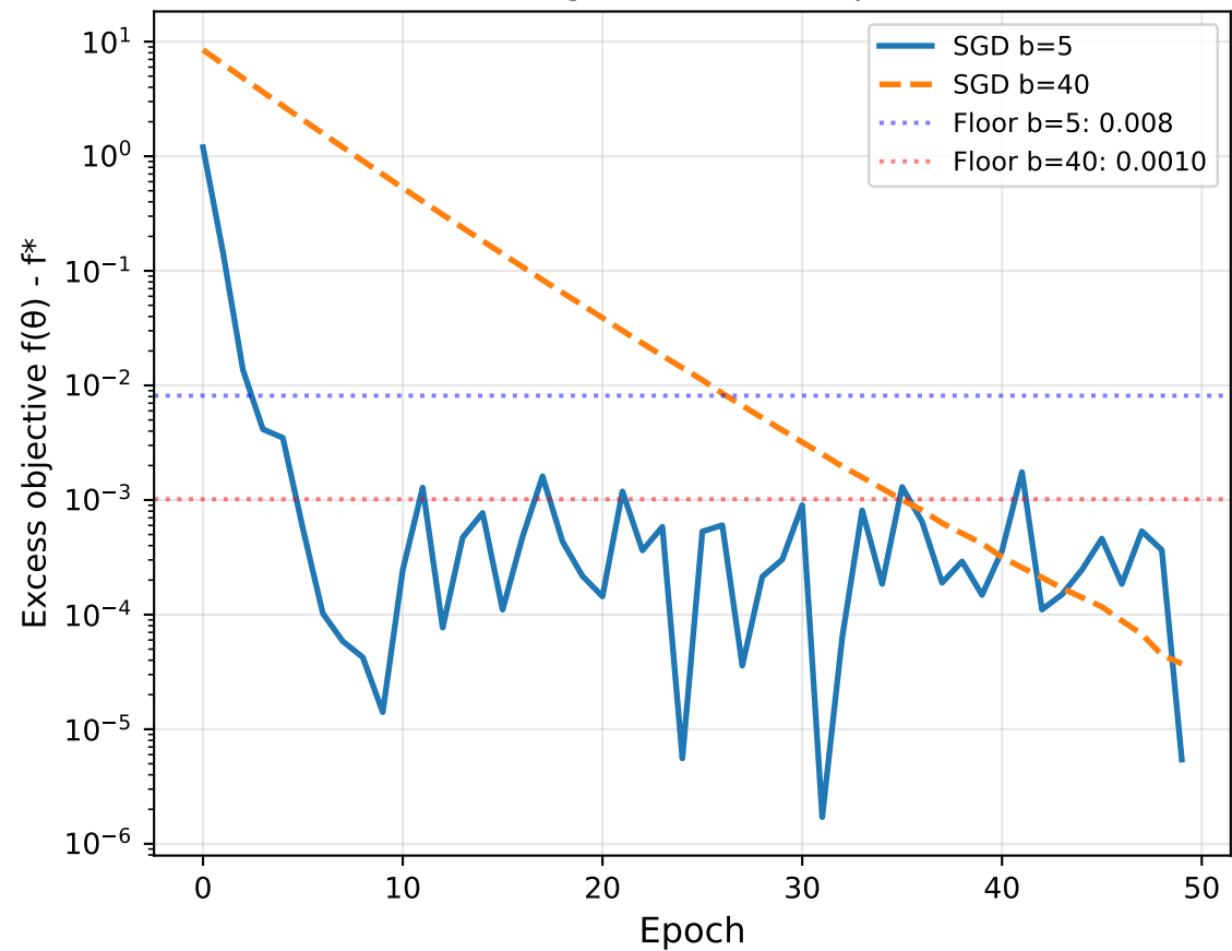
SGD convergence ( \sigma=1.0 , Prop. 2 floor)
