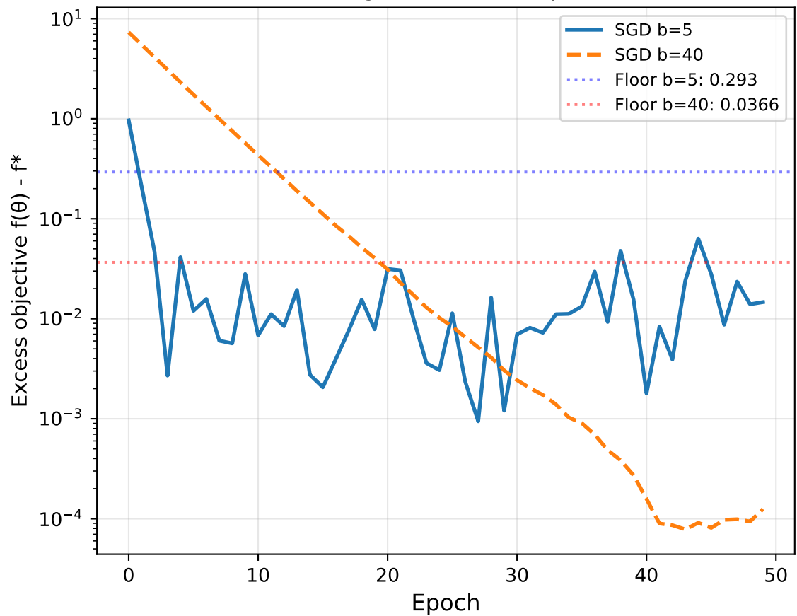
SGD convergence ( \sigma=6.0 , Prop. 2 floor)
