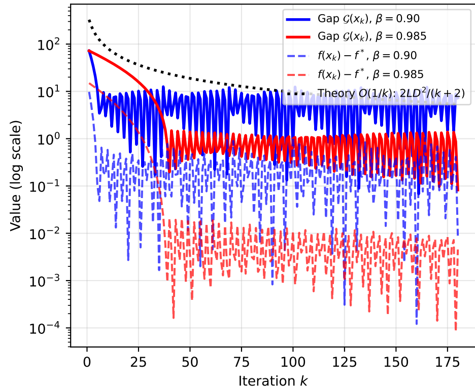
Interior opt.: FW gap vs suboptimality
