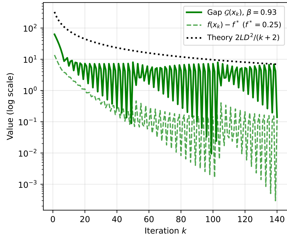
Boundary opt.: FW gap (loose at boundary)
