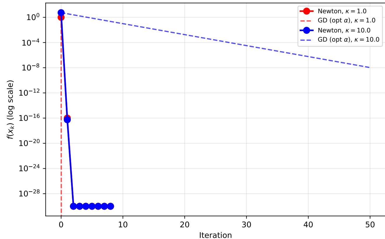
Newton (quadratic rate) vs GD (linear rate) (quadratic losses, x_0 = (1, 1) )
