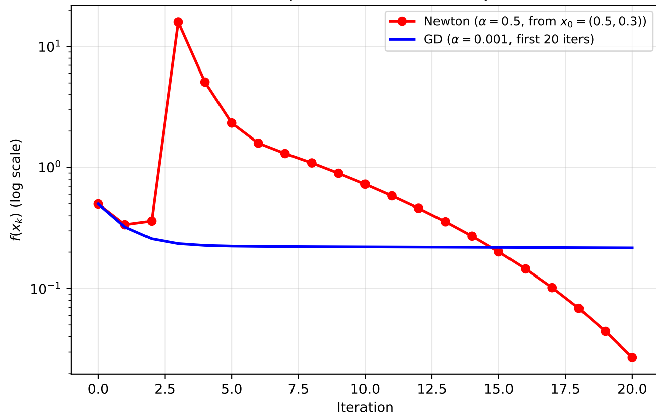
Newton's Rapid Convergence on Rosenbrock (near-optimum start for visibility)
