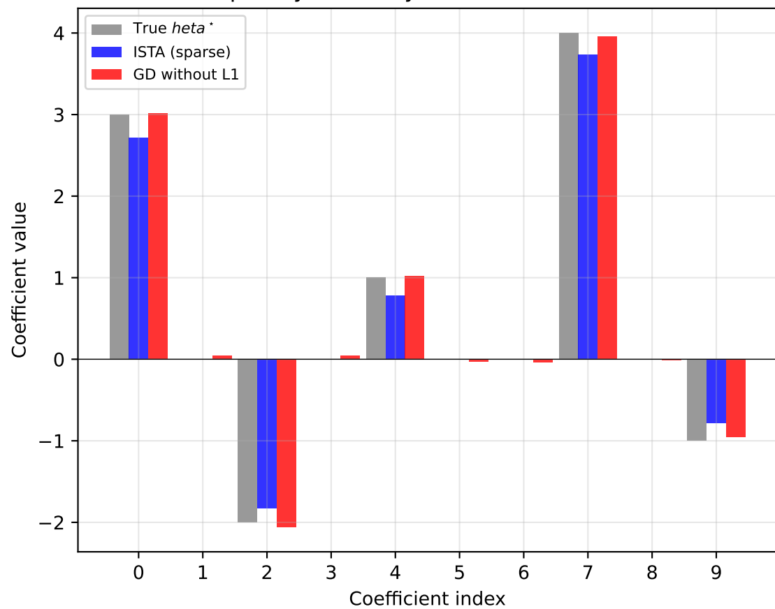
Sparsity Recovery: LASSO vs Plain GD
