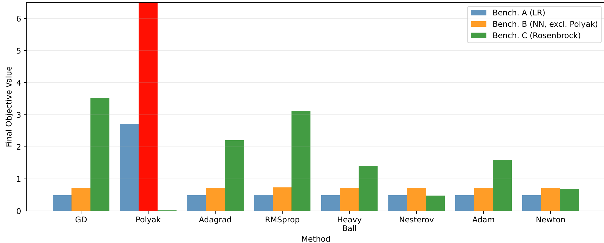
Final Objective Values by Method and Benchmark (Q1: 120 iters; Q2: 150 iters; Newton: 20 iters)
