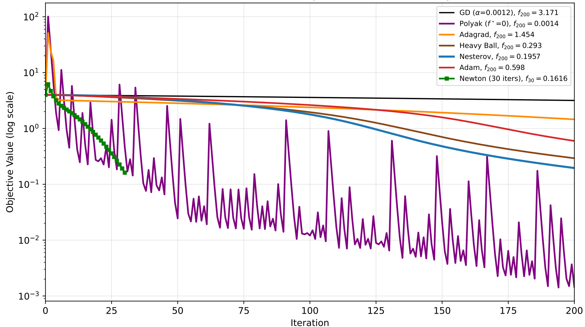
Benchmark C (Rosenbrock): Comprehensive Method Comparison
