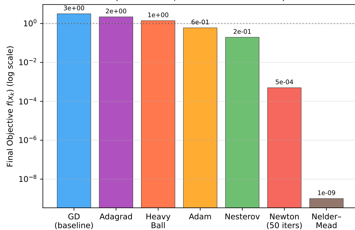
Final Objective on Rosenbrock (All Methods, 200 Iterations or Less)
