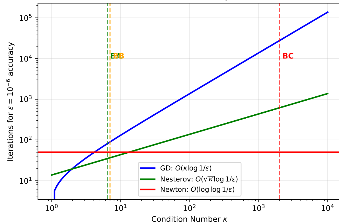
Algorithm Complexity vs Condition Number ( \epsilon = 10^{-6} accuracy)
