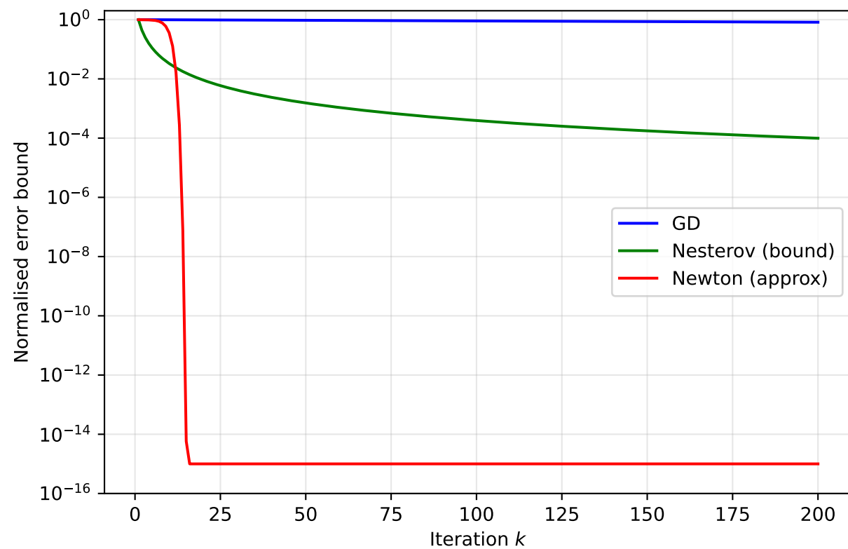
Convergence Rate Comparison ( \kappa = 2000 ) Normalised to initial error
