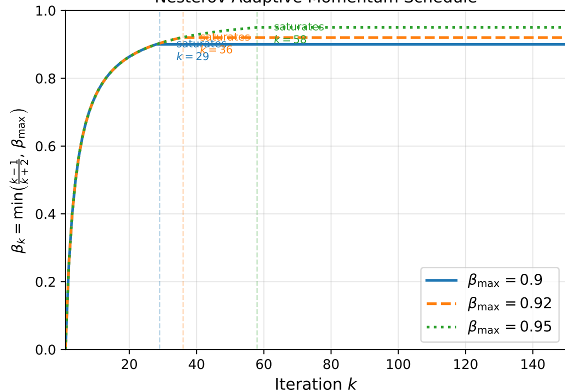
Nesterov Adaptive Momentum Schedule
