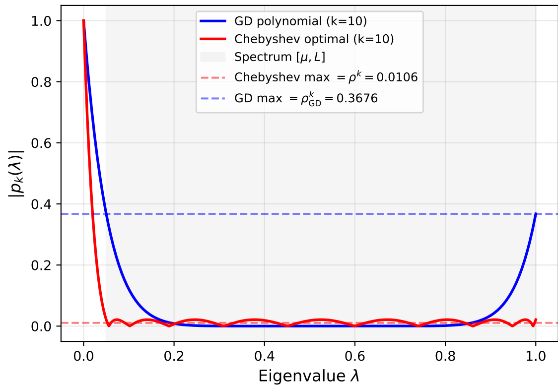
Chebyshev vs GD Polynomial ( k=10, \kappa=20 )
