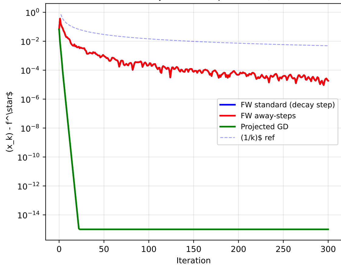
FW vs Proj-GD on Simplex (=20$)
