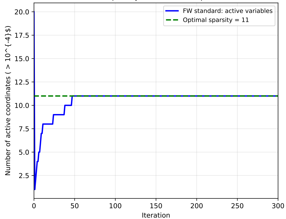
FW Sparsity Evolution (Simplex)
