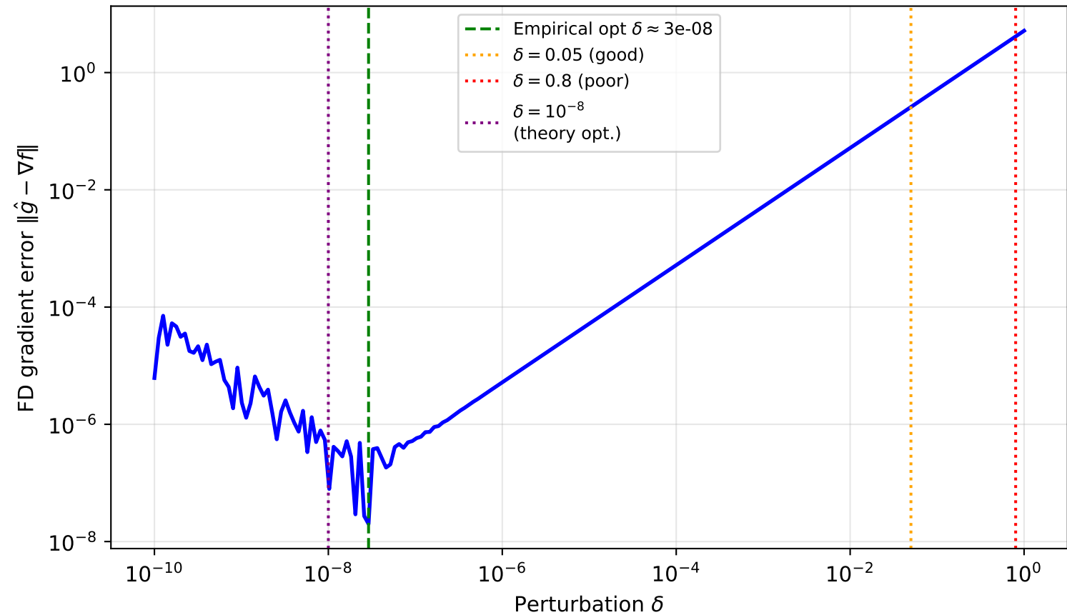
Forward FD gradient error vs \delta at x_0 = (-1, 4) , Benchmark B
