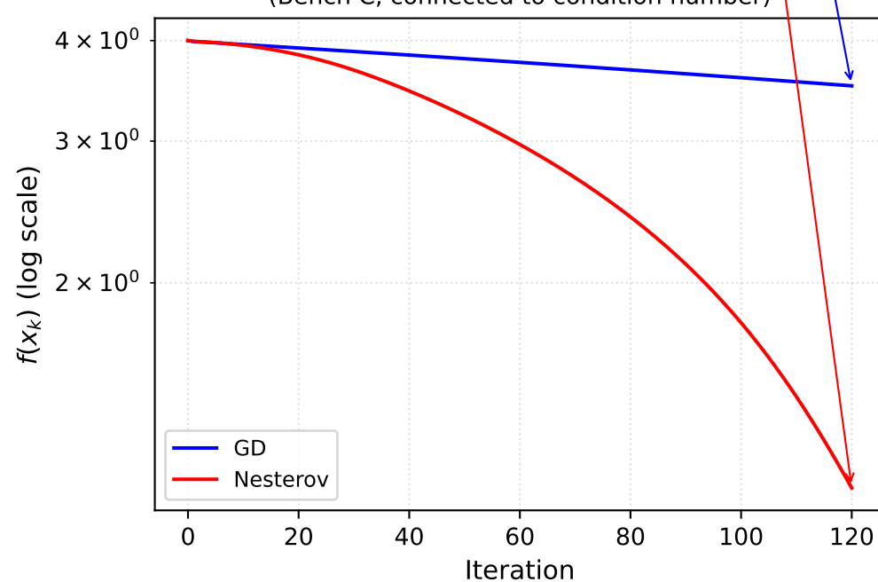
Objective convergence: GD vs Nesterov (Bench C, connected to condition number)
