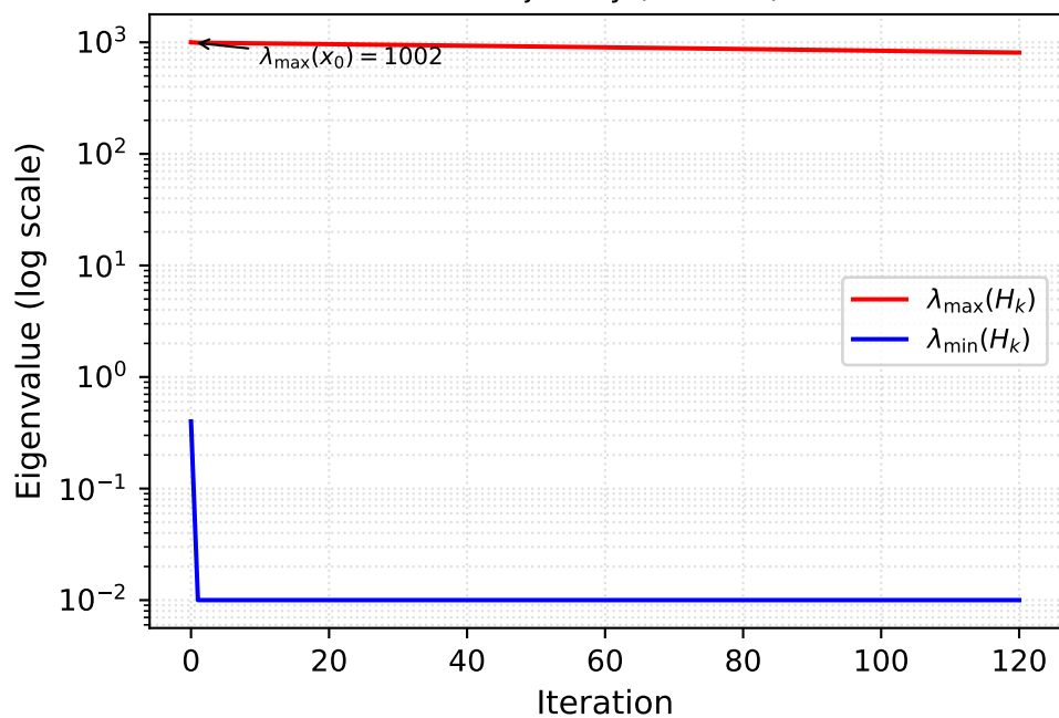
Hessian eigenvalues along GD trajectory (Bench C)
