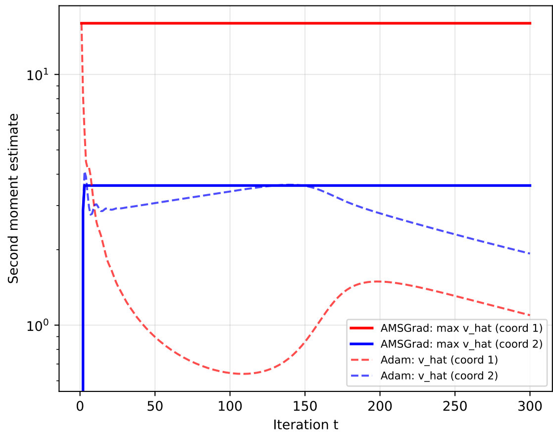
Adam vs AMSGrad: Second Moment Estimates
