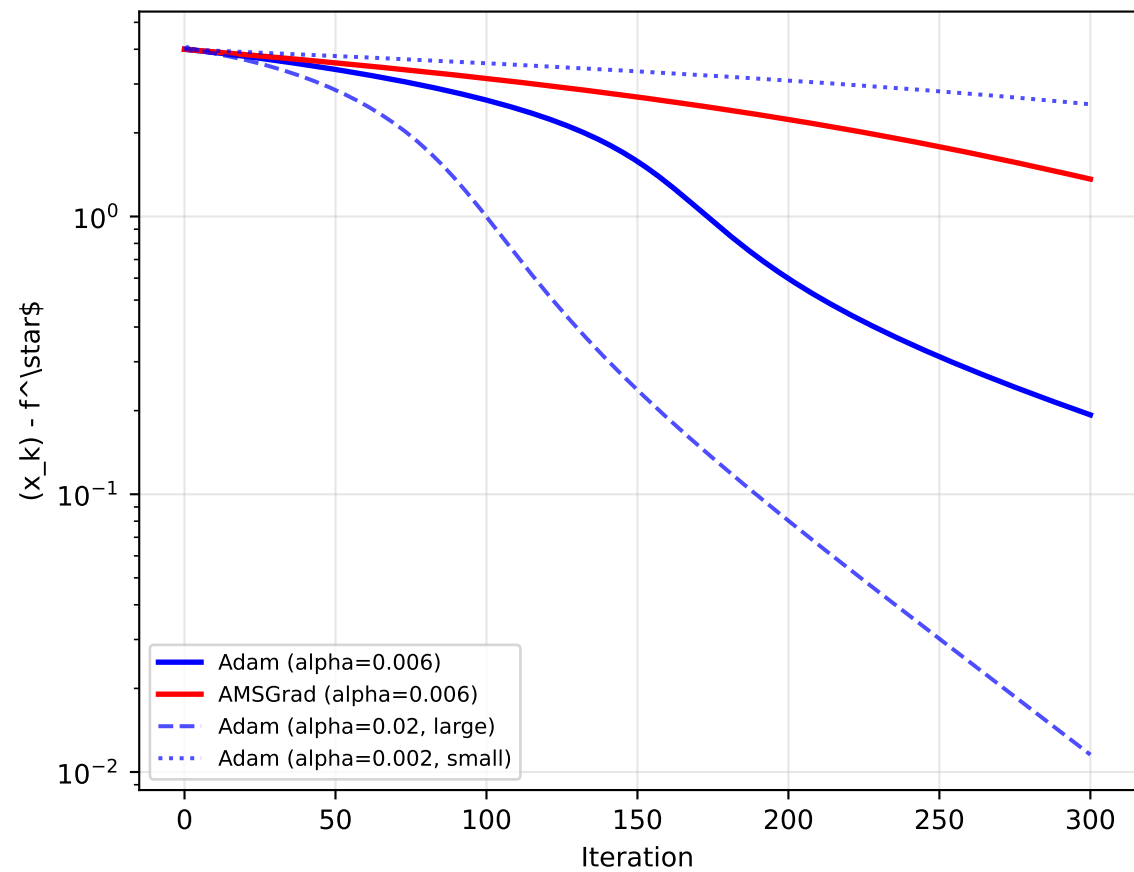
Adam vs AMSGrad: Rosenbrock (300 iters)
