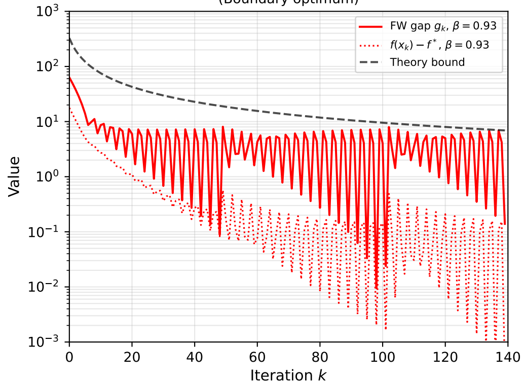
FW gap vs suboptimality (Boundary optimum)
