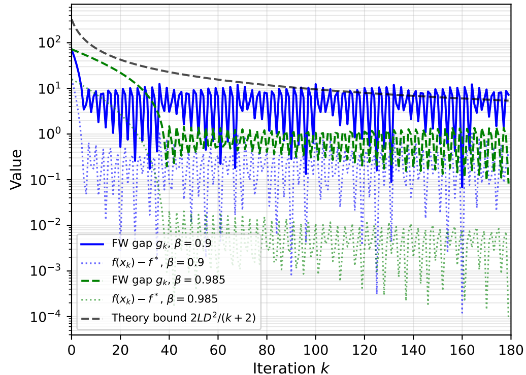
FW gap vs suboptimality (Interior optimum)
