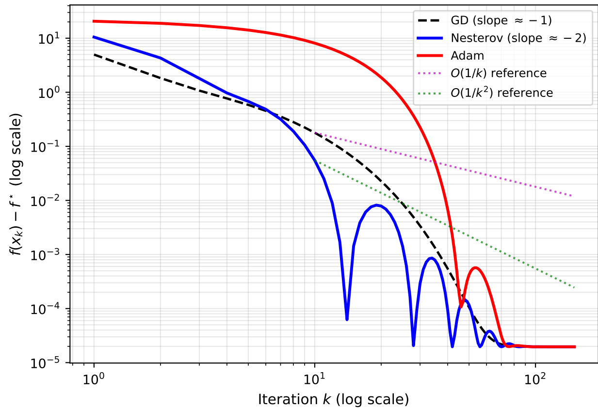
Q2: Convergence Rate on Benchmark B (log-log: slope = convergence order)
