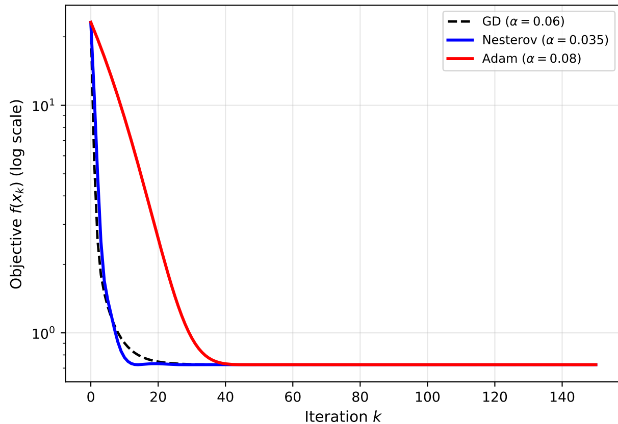
Q2: Convergence on Benchmark B (standard semi-log)
