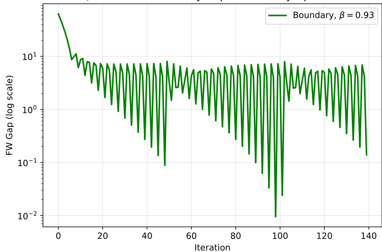
Q6: Frank-Wolfe Duality Gap — Boundary Optimum
