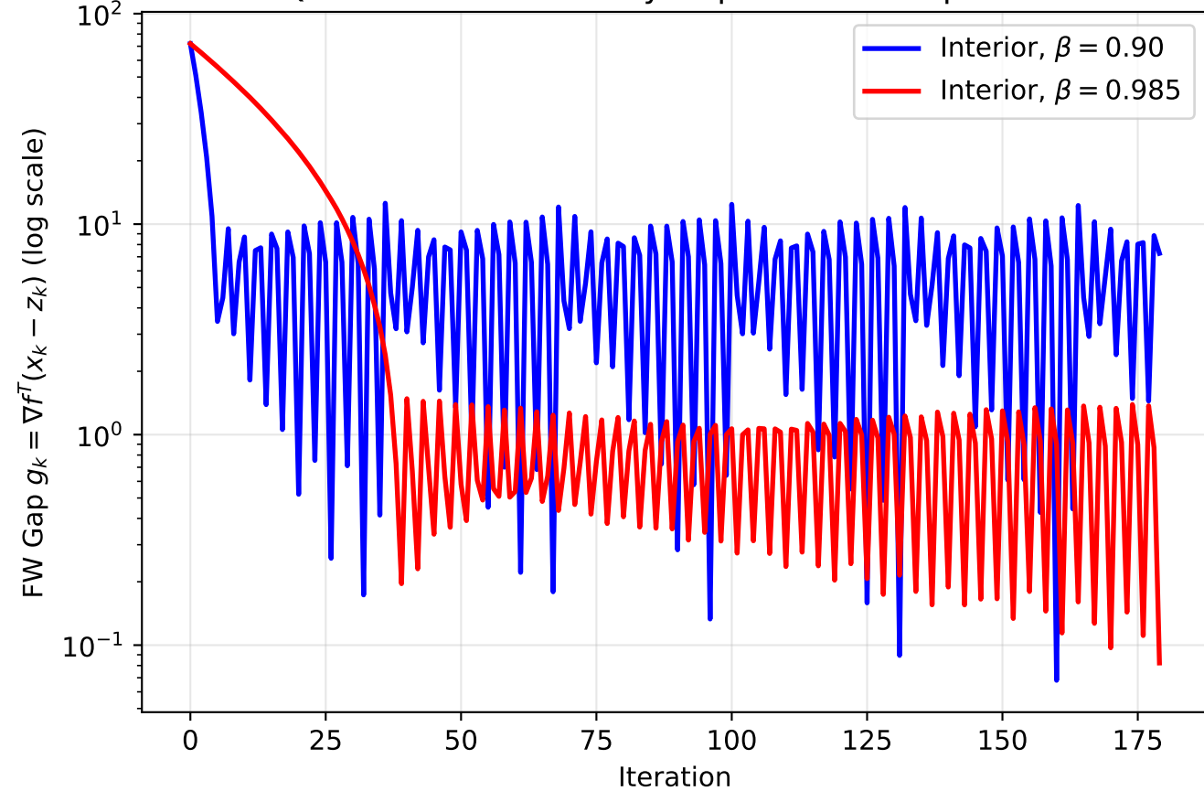
Q6: Frank-Wolfe Duality Gap — Interior Optimum
