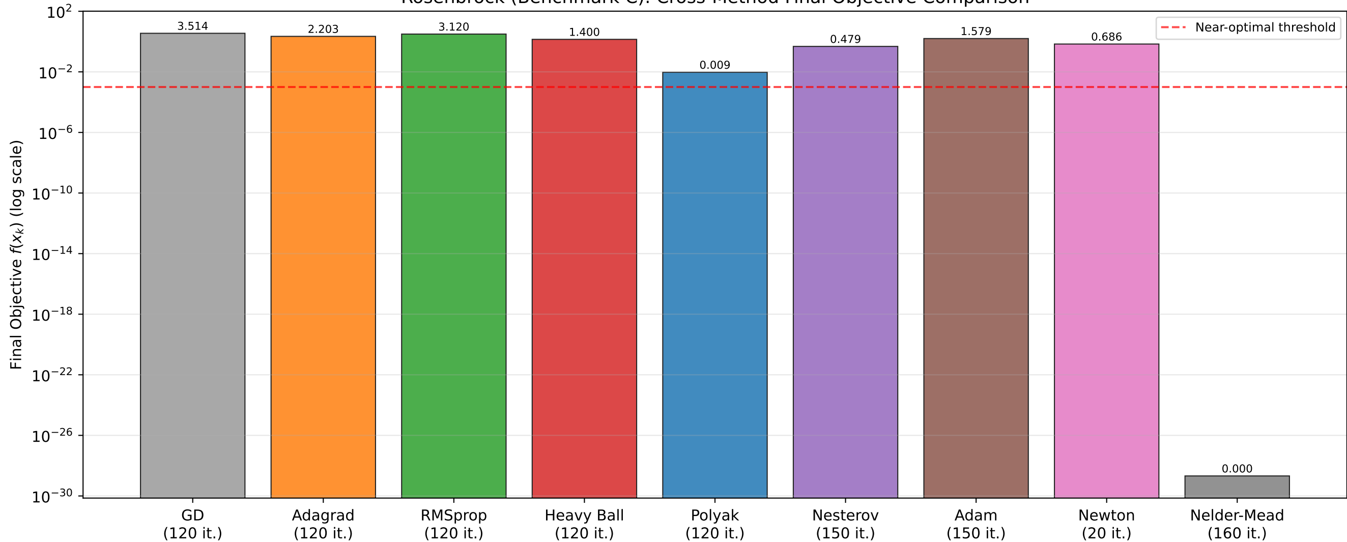
Rosenbrock (Benchmark C): Cross-Method Final Objective Comparison
