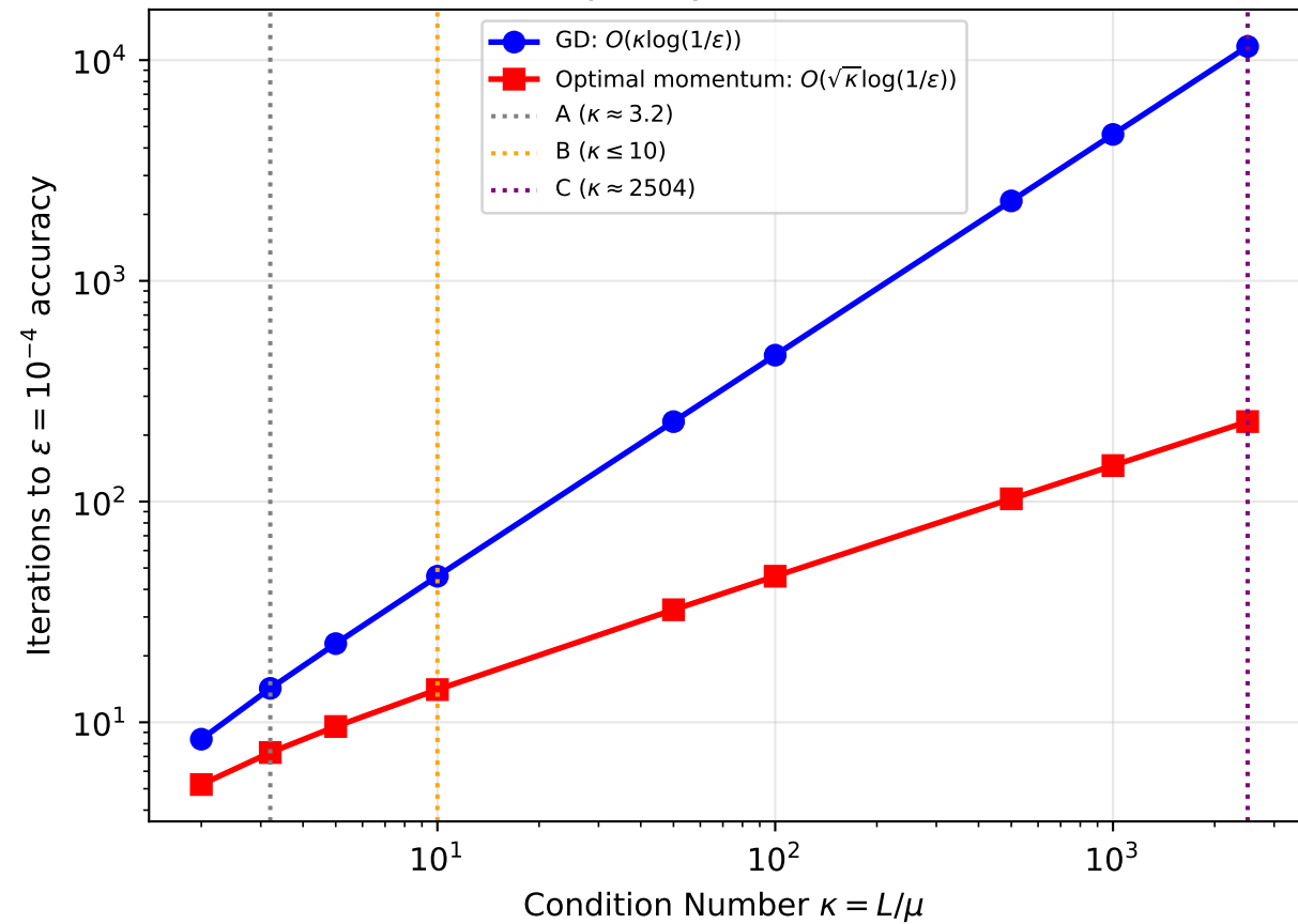
Iteration Complexity vs Condition Number
