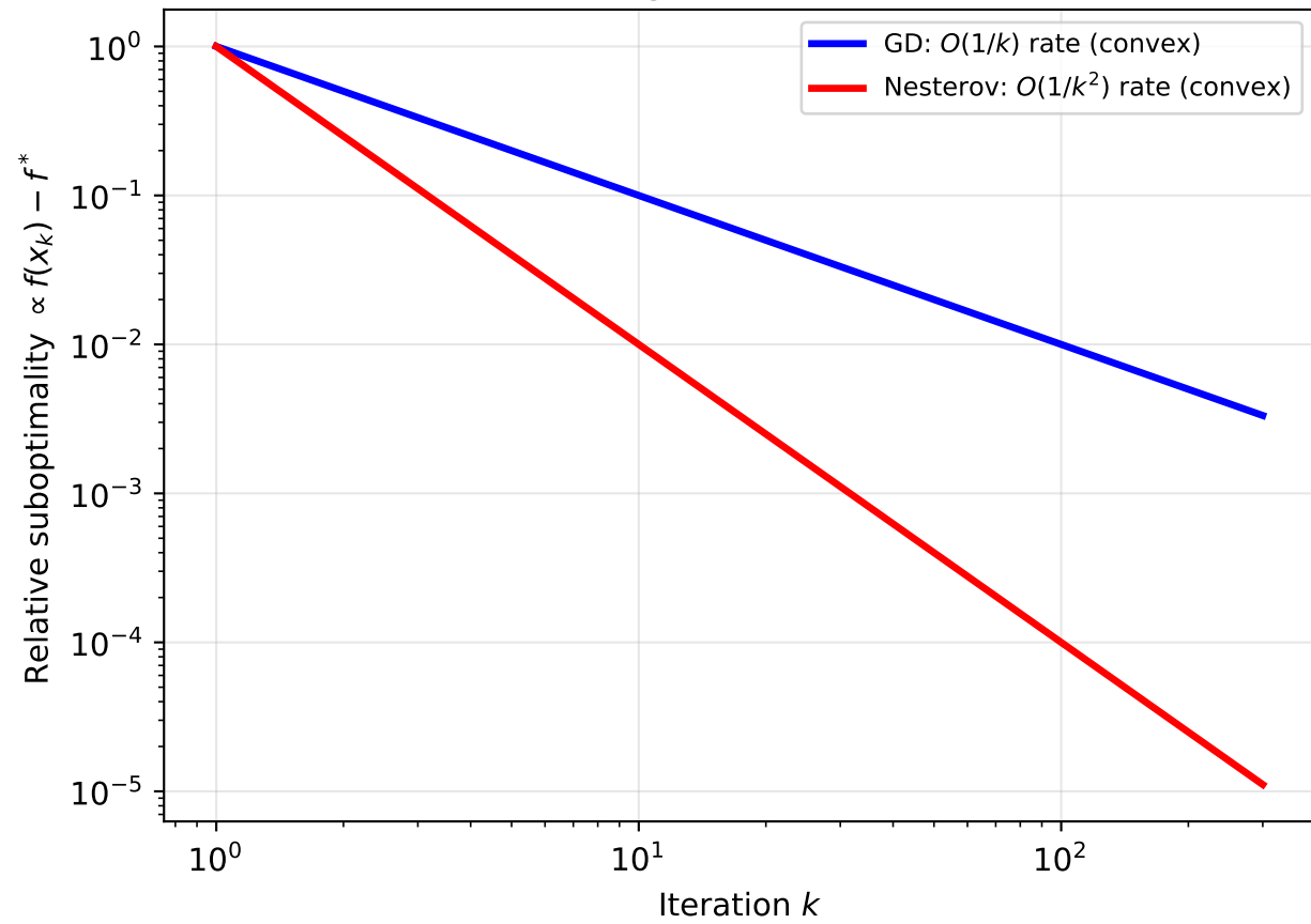
Theoretical Convergence Rates: GD vs Nesterov
