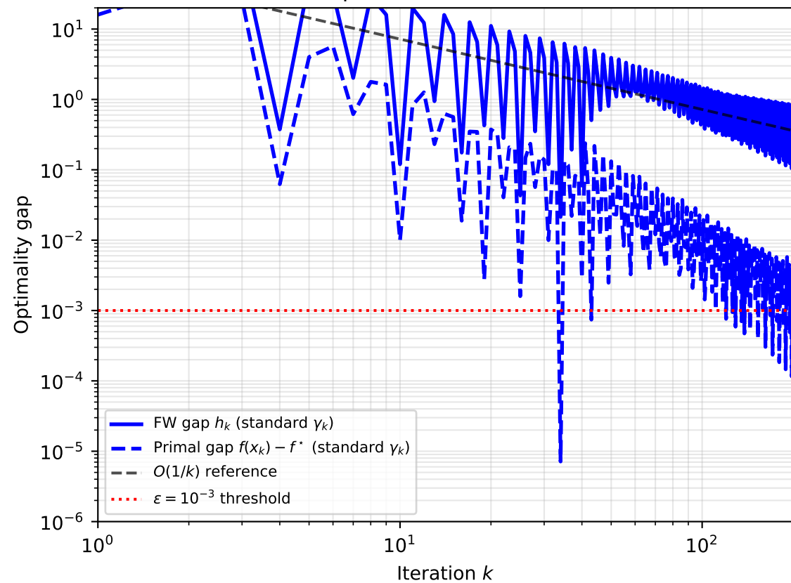
FW Gap as Stopping Criterion (Interior optimum, standard schedule)
