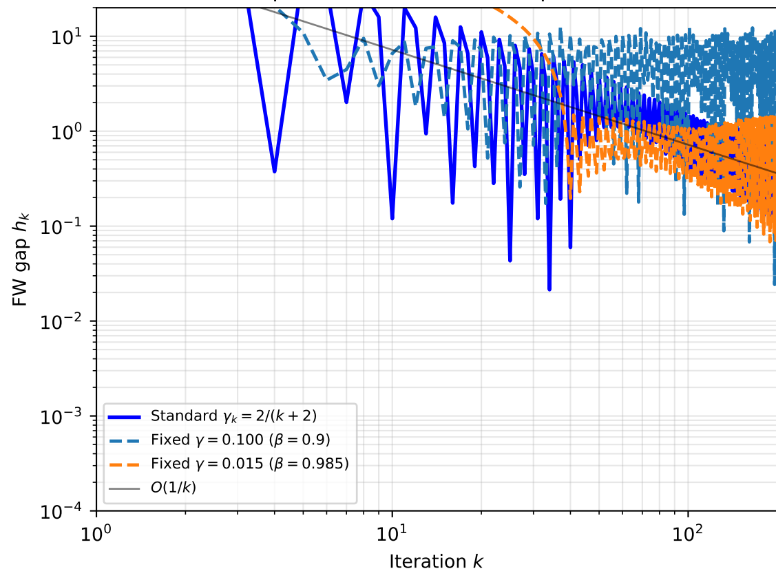
FW Gap: Standard vs Fixed Step Schedules
