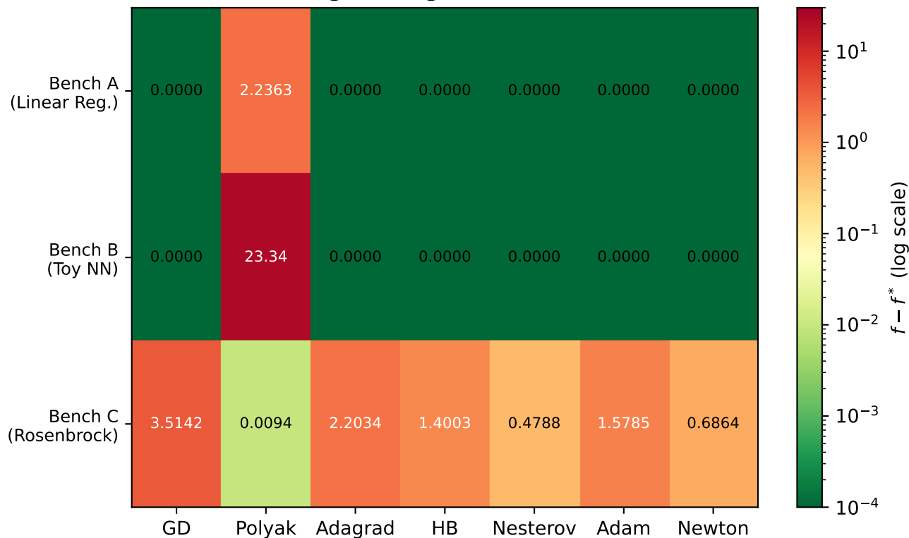
Excess Above Optimum f(x_k) - f^* (log scale, green=better)
