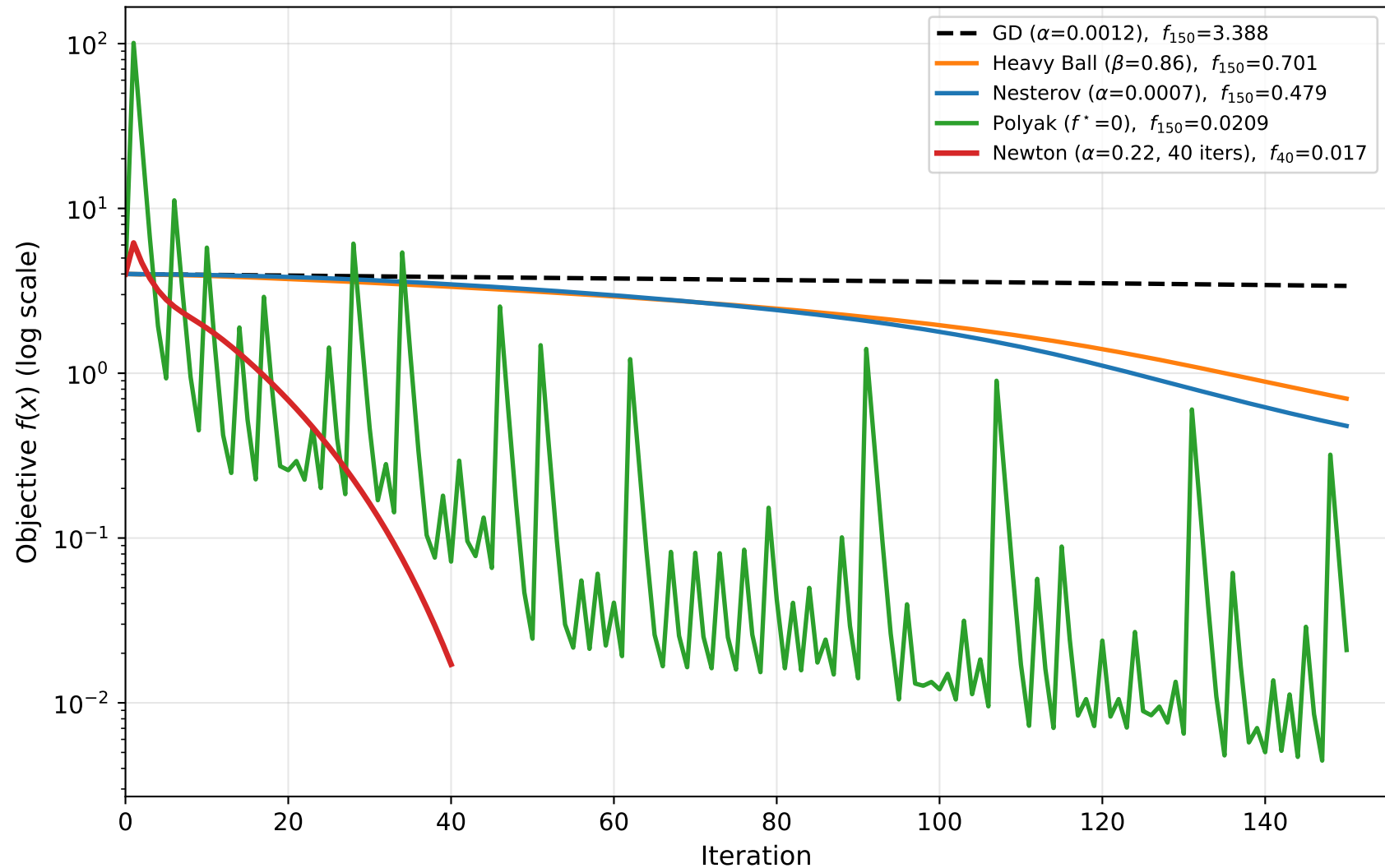
Convergence Comparison Across All Methods — Benchmark C (Rosenbrock)
